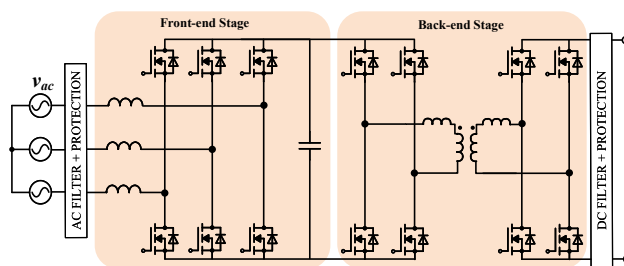
Fig. 1. Example of a two-stage high power OBC configuration suitable to G2V and V2G charging
