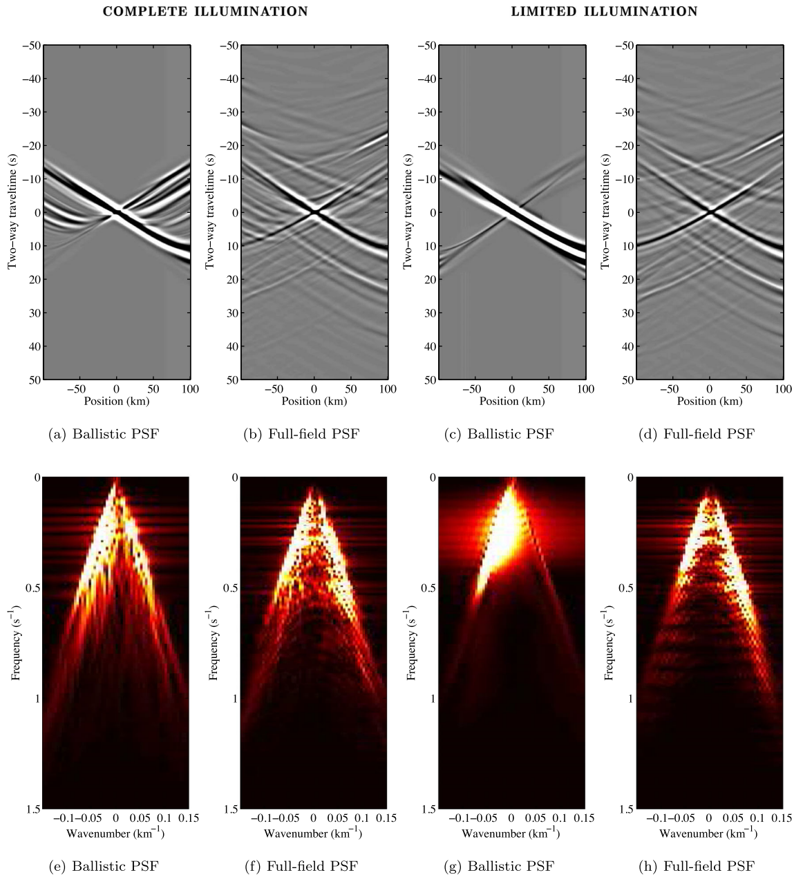
Figure 5. Ballistic and full-field PSF's of the virtual source at position 0 km for the complete (Fig. 3a) and limited (Fig. 4a) illumination scenarios. (a) Ballistic PSF in the t - x domain for complete illumination. (b) Full-field PSF in the t - x domain for complete illumination. (c) Ballistic PSF in the t - x domain for limited illumination. (d) Full-field PSF in the t - x domain for limited illumination. (e)–(h) show the f - k spectra of (a)–(d).
