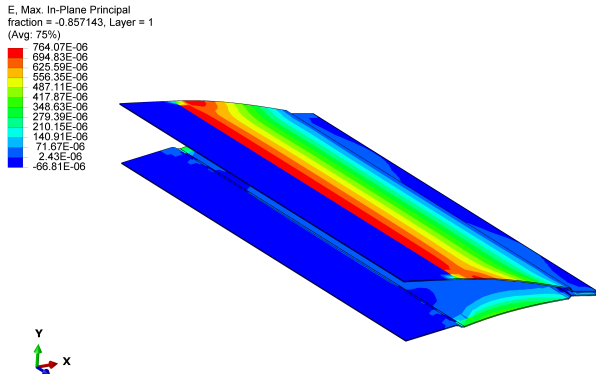
FIGURE 19. STRAIN IN TOP SKIN AT MAXIMUM DEFLECTION.
