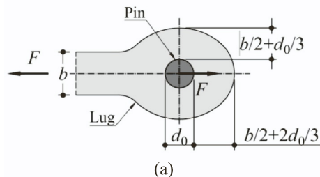
Fig. 2. Lug geometry: (a) adapted from Winkler; (b) adapted from EC3-1-8 ('Type A' geometry).
