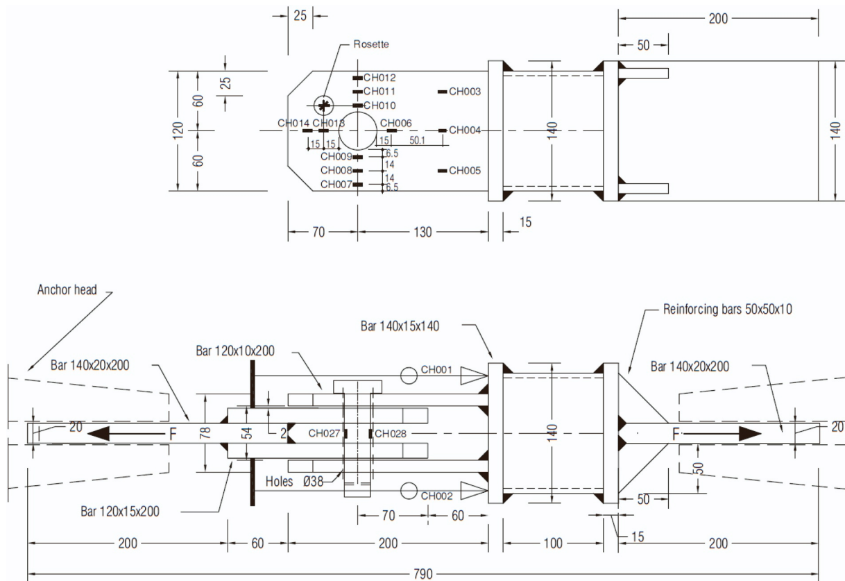
Fig. 10. Instrumentation of the laboratory models: exemplification for Prototype 1 with \phi 36 mm pin.
