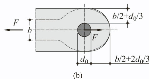
Fig. 2. Lug geometry: (a) adapted from Winkler; (b) adapted from EC3-1-8 ('Type A' geometry).
