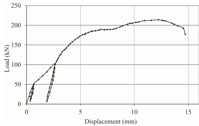
Fig. 16. Force-displacement curve for Prototype 2.
