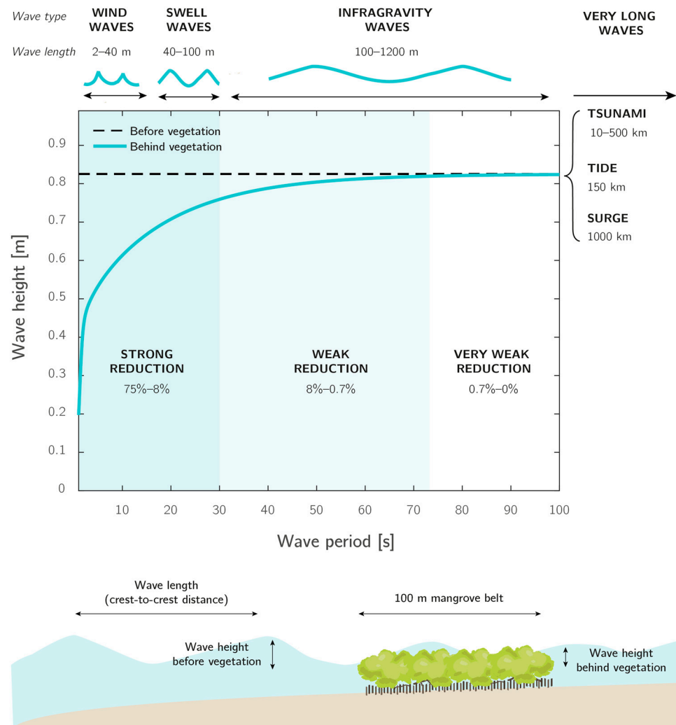
Figure 3. Diagram illustrating the amount of wave reduction for a fixed value of incoming wave height and varying wave periods through a 100 m-wide mangrove belt. The diagram was derived using the model of Mendez and Losada [28] with mangrove vegetation parameters obtained from Suzuki [29]; vegetation density of 1.1 trees/m 2 and tree diameter of 0.27 m. The results were obtained with a water depth of 1.5 m and a wave height of 0.8 m (maximum wave height possible with a breaking ratio of 0.55). The wave lengths indicated in the figure were also calculated for a water depth of 1.5 m.
