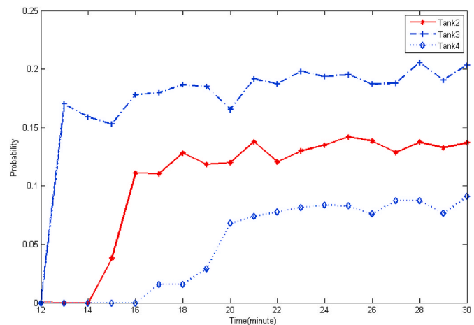
Fig. 9. Fire probabilities of tanks over time.
