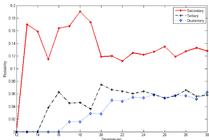
Fig. 10. Probabilities of domino effect level over time.
