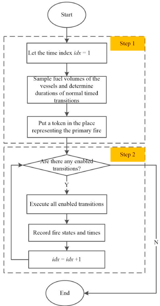
Fig. 2. Main flowchart of a simulation.
