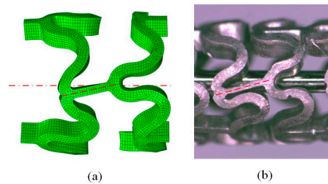
Figure 13. Comparison between (a) simulated and (b) experimental profiles of crimped Stent A.
