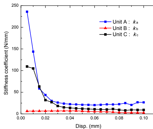
Figure 8. Displacement-dependent stiffness coefficients, k_a , k_b , and k_c , of the single unit of Patterns A, B, and C, respectively.
