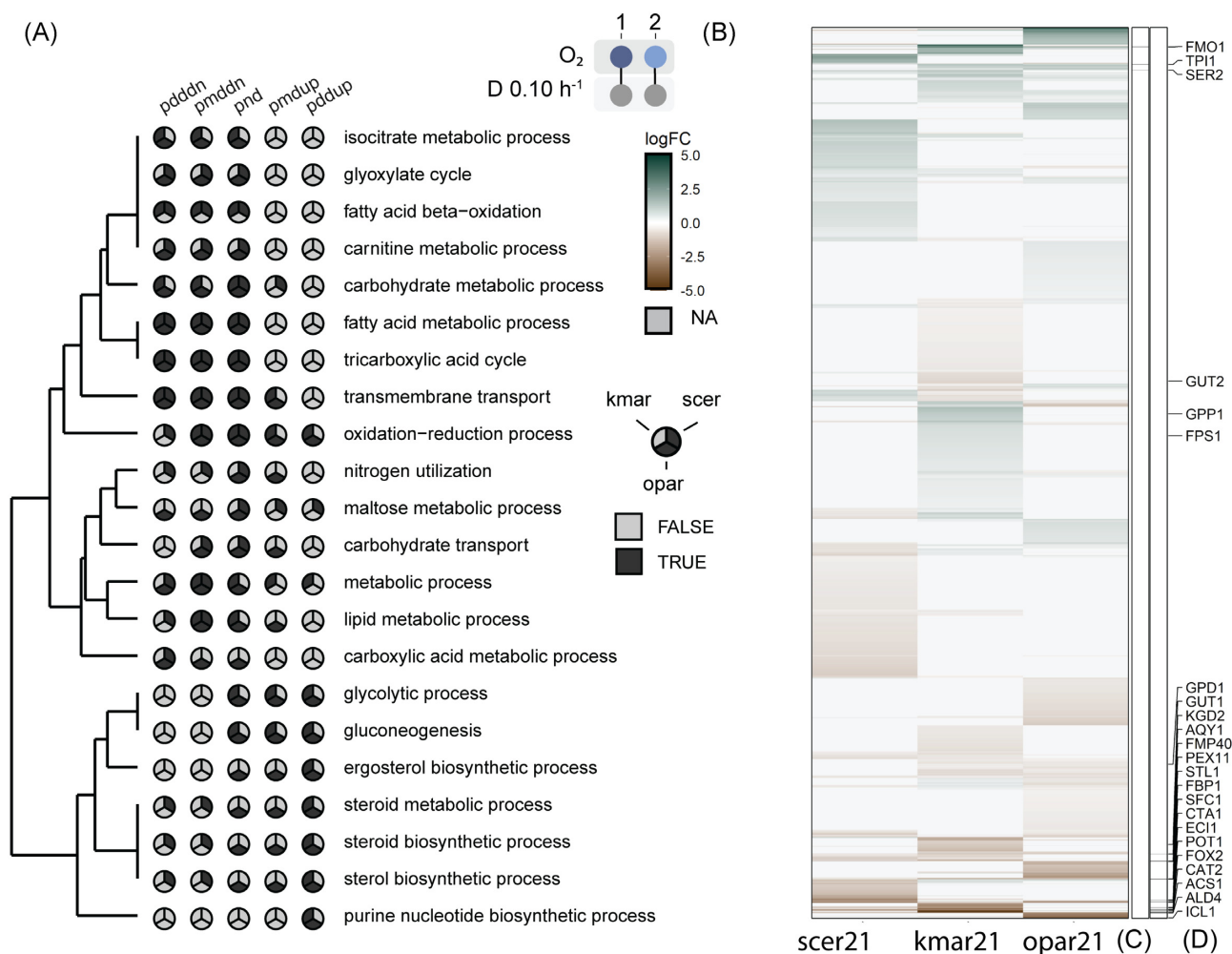
Figure 2. Genome-wide transcriptional responses of O. parapolyomorpha ( opar ), K. marxianus ( kmar ), and S. cerevisiae ( scer ) to oxygen limitation. Aerobic (regime 1, 21 \times 10^4 ppm O_2 in inlet gas, and 7.5 \text{ g l}^{-1} glucose in feed medium) and oxygen-limited (regime 2, 840 ppm O_2 in inlet gas; 20 \text{ g l}^{-1} glucose in feed medium) chemostat cultures were grown at D = 0.1 \text{ h}^{-1} and 30^\circ\text{C} . Data for K. marxianus and S. cerevisiae were obtained from a previous study (Dekker et al. 2021). (A) Gene-set enrichment analysis showing GO-terms overrepresented among genes showing a transcriptional response to oxygen limitation (regime 2 versus regime 1) in at least two of the three yeast species. Distinct directionalities calculated with Piano (Våremo et al. 2013) are indicated as distinct-directional down (pdddn), mixed-directional down (pmddn), nondirectional (pnd), mixed-directional up (pmdup), and distinct-directional up (pddup). Hierarchical clustering was based on degree of overrepresentation. Data on all enriched GO-terms for biological processes are shown in Figures S2–S4 (Supporting Information). (B) Log-fold changes (regime 2 versus regime 1) of orthologs in the three yeasts, (C) Orthologs showing higher transcript levels in oxygen-limited cultures of all three yeasts, (D) Orthologs showing lower transcript levels in oxygen-limited cultures of all three yeasts.
