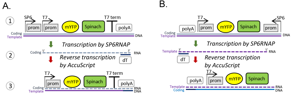
Figure 5.6: Scheme of the stepwise production of templates resulting in DNA template :RNA coding (A) or RNA template :DNA coding hybrids (B). The use of the SP6 RNAP for the transcription step enables the inclusion of a functional T7 promoter in the final template (or vice versa). C) The hybrid template is imaged on an agarose gel together with the starting double stranded DNA, the intermediate RNA, a control sample, DNA (left) and RNA ladders (right) .
