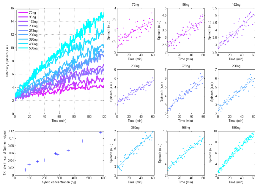
Figure 5.17: Linear fits of the first 60 min of the Spinach transcription signal for all the curves analyzed for the T7D templates and displayed in the main panel.
