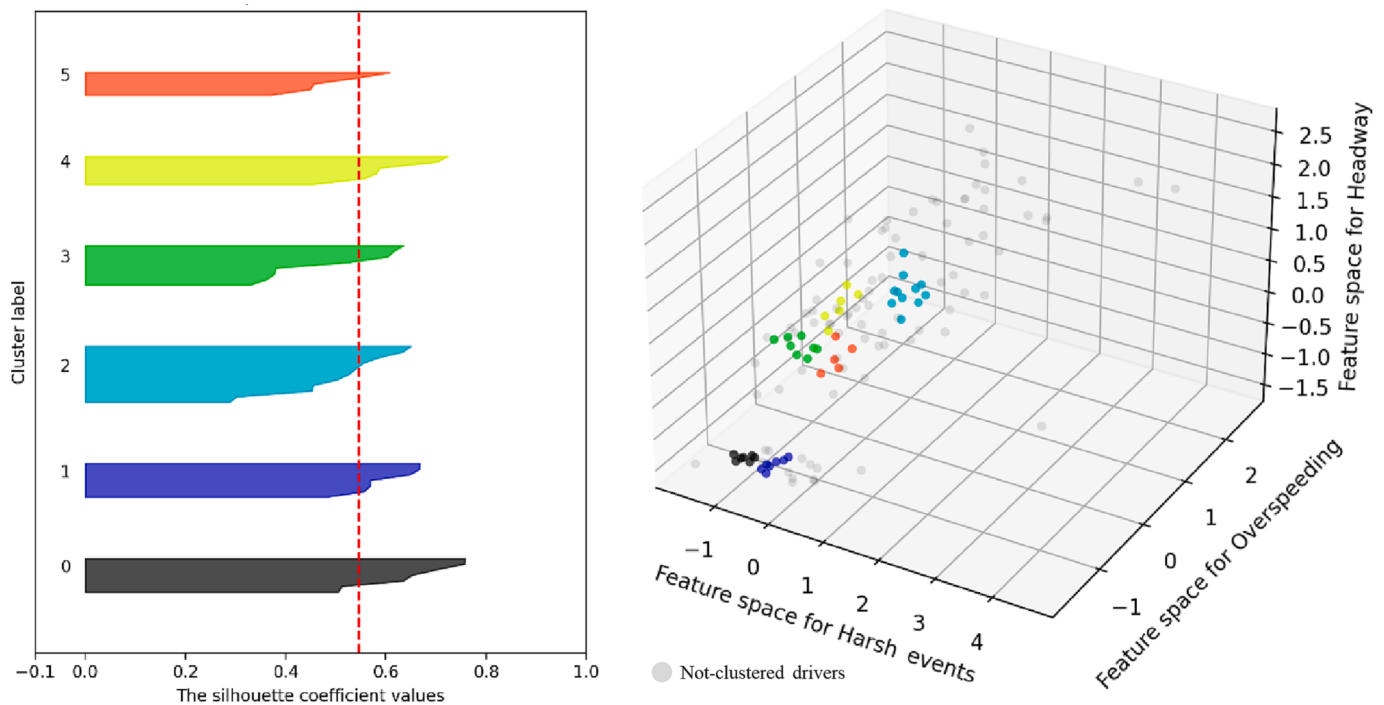
Fig. 9. Results of the OPTICS 6-cluster clustering. (a) Silhouette plot for all clusters; (b) 3D illustration of the 3 normalized features used in clustering.
