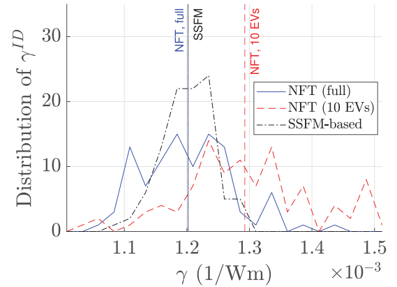
Fig. 2. Distribution of the identified \gamma from raised cosine bursts with vanishing tails.
