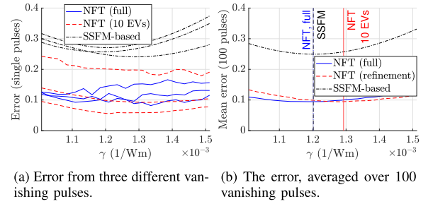
Fig. 5. Error-curves of the SSFM-based method and the NFT-based methods for the raised cosine pulse with vanishing tails, from Section V-B and Fig. 2.
