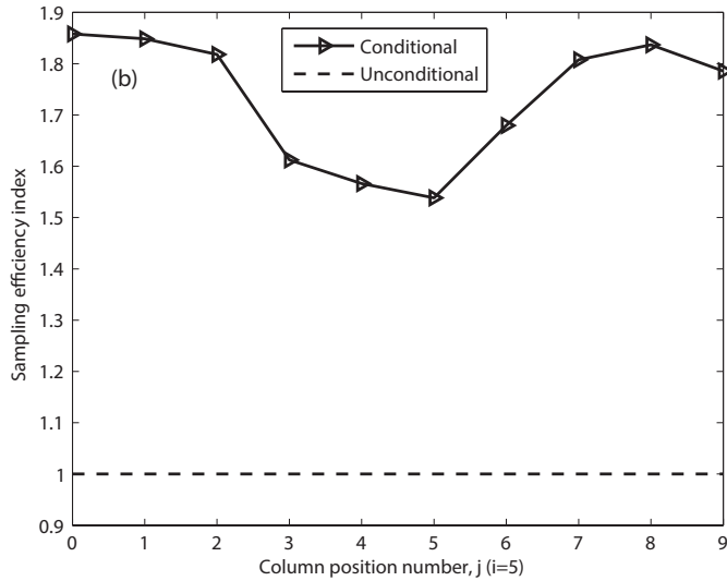
Figure 6.12: Influence of CPT location j during the second phase of site investigation (based on \theta_v = 1.0 m and 500 realisations per simulation): probability density function of realised factor of safety ( \xi = 6 ) (a); influence of CPT location j with i = 5 ( \xi = 6 ) (b)
