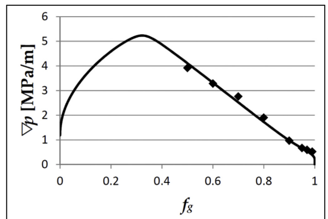
Fig. 6. Steady state f_g vs. \nabla p data for the experiment using the APG surfactant along with STARS model fit using the following parameter values: fmmob = 20 , fmdry = 0.59 \pm 0.01 , epdry = 600 .
