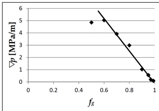
Fig. 7. Steady state pressure gradient \Delta p over the middle section of the core for the experiment using the AES surfactant as a function of foam quality ( f_g ). All data points except the lowest foam quality studied ( f_g = 0.5 ) are clearly in the high-quality regime. Straight line fit is first estimate and is used to determine limiting water saturation S_w^* .
