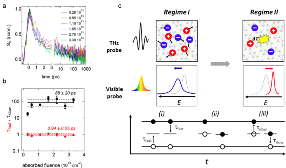
Figure 5. (a) Normalized decay traces of the real part of the THz conductivity, a metric for the charge population, for increasing absorbed photon density ( 0.28 \times 10^{13} – 3.3 \times 10^{13} \text{cm}^{-2} ). (b) Time constants extracted from a biexponential fit to (a) showing density-independent recombination dynamics for both fast (red, \tau_{\text{fast}} = 0.94 ps) and slow (black, \tau_{\text{slow}} = 88 ps) timescales. (c) Schematic summary representation of the proposed charge carrier generation and decay in liquid-phase exfoliated \text{ReS}_2 , proceeding through two distinct regimes. An optical pump generates predominantly free mobile charge carriers, as evidenced by THz spectroscopy, that initially cause broadening and a blueshift of the exciton profile due to collisional broadening and free carrier screening, respectively. Next, the broadened and blue-shifted transition decays into a peculiar narrowed, and red-shifted line profile on a similar timescale as the THz conductivity decays. The latter indicates a nonradiative recombination event giving rise to the observed spectral signatures, i.e. , a redshift due to heating or carrier-capture-induced energetic redshifts and a narrowing due to a homogenization of the energy landscape.
