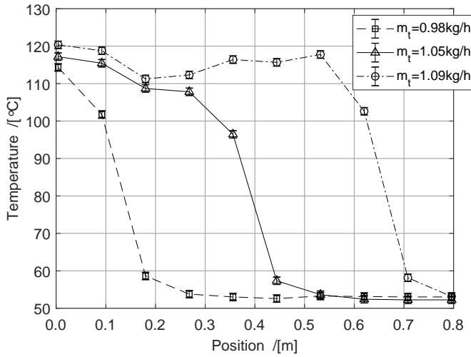
Figure 3.10: Temperature results from the sensors located along the shell side of the mini-channel heat exchanger when the shell side mass flow is fixed at 7.5 kg/h for the NH 3 -H 2 O experiments. Error bars are included (see section 2.2 for details). The lines serve as visual guidelines for the reader.
