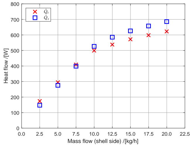
Figure 3.5: Heat flow of the shell side, \dot{Q}_s , and tube side, \dot{Q}_t , for the water-water experiments.
