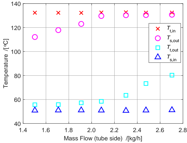
Figure 3.16: The in- and outlet temperatures for the \text{NH}_3\text{-CO}_2\text{-H}_2\text{O} experiments at various tube side mass flows when the shell side mass flow is kept constant at 5 kg/h.
