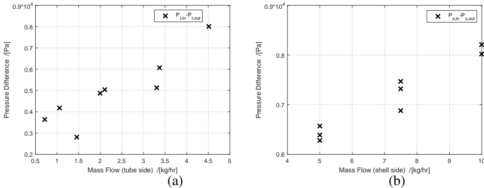
Figure 3.17: Pressure drop over the mini-channel heat exchanger on the tube side ( \text{NH}_3\text{-CO}_2\text{-H}_2\text{O} side) (a), and the shell side (water side) (b).
