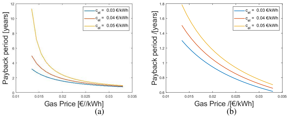
Figure 5.10: The simple payback period as a function of the gas and electricity price for a compressor outlet vapor quality of 0.5 and \text{NH}_3 concentration of 0.55, when waste heat stream is heated from 90 to 130 °C, assuming 5 MW thermal output. Not taking into account the cost of \text{CO}_2 (a), taking into account the cost of \text{CO}_2 (b)
