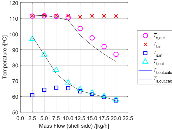
Figure 3.7: In- and outlet temperatures for the water-water experiments. The tube side mass flow is kept constant at 10 kg/h while the shell side mass flow ranges from 2.5 to 20 kg/h. The markers are the experimental values while the solid lines are calculated with the method proposed by Nefs et al. [74] and discussed above.
