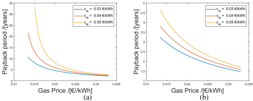
Figure 5.11: The simple payback period as a function of the gas and electricity price for a compressor outlet vapor quality of 0.6 and \text{NH}_3 concentration of 0.65, when waste heat stream is heated from 60 to 140 °C, assuming 5 MW thermal output. Not taking into account the cost of \text{CO}_2 (a), taking into account the cost of \text{CO}_2 (b)
