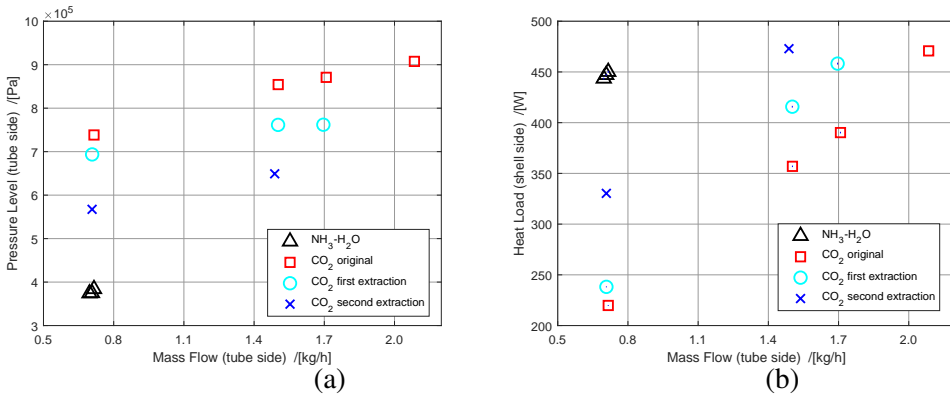
Figure 3.21: Results for a shell side mass flow of 5 kg/h before and after draining of the mixture with added \text{CO}_2 compared to the \text{NH}_3\text{-H}_2\text{O} results, the different pressure levels (a), and the shell side heat load (b). It is clear that comparable pressure levels were not reached with the added \text{CO}_2 . However, with each extraction the performance at similar mass flows approached the performance of the \text{NH}_3\text{-H}_2\text{O} mixture.
