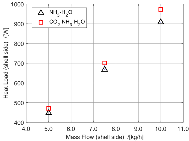
Figure 3.18: Shell side heat load for the NH 3 -H 2 O and NH 3 -CO 2 -H 2 O experiments.
