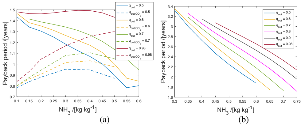
Figure 5.7: The simple payback time taking the cost of \text{CO}_2 into account as a function of the \text{NH}_3 concentration for various compressor outlet vapor qualities, assuming 5 MW thermal output, when a waste heat stream is heated from 90 to 130 °C (a) and from 60 to 140 °C (b). The solid lines are the results for \text{NH}_3\text{-H}_2\text{O} and the dotted lines with added 5 wt% \text{CO}_2 .
