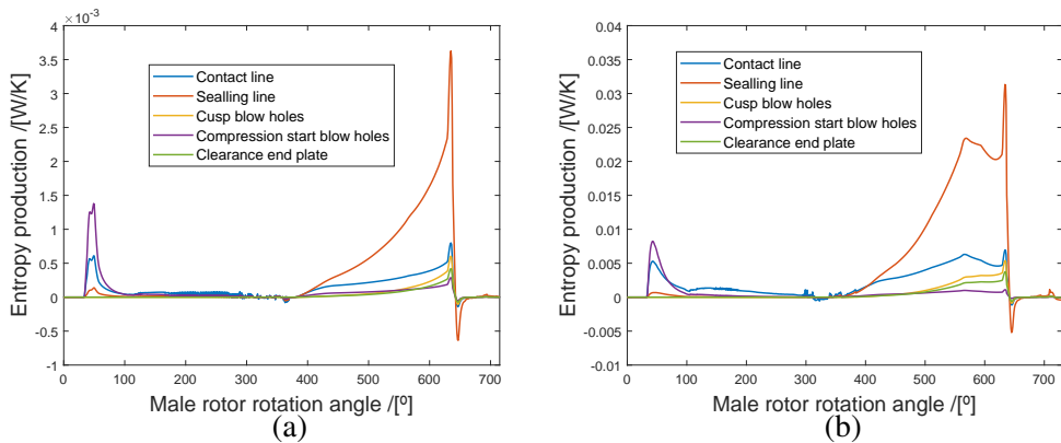
Figure 4.4: \dot{\sigma} for each leakage path in the compressor, 10 \mu\text{m} (a) and 100 \mu\text{m} (b).
