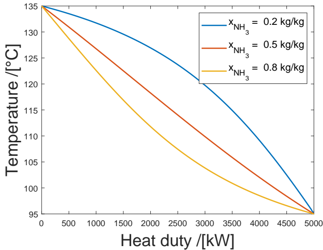
Figure 5.9: Example temperature glides as a function of the heat load for NH 3 concentrations of 0.2 kg/kg, 0.5 kg/kg and 0.8 kg/kg.
