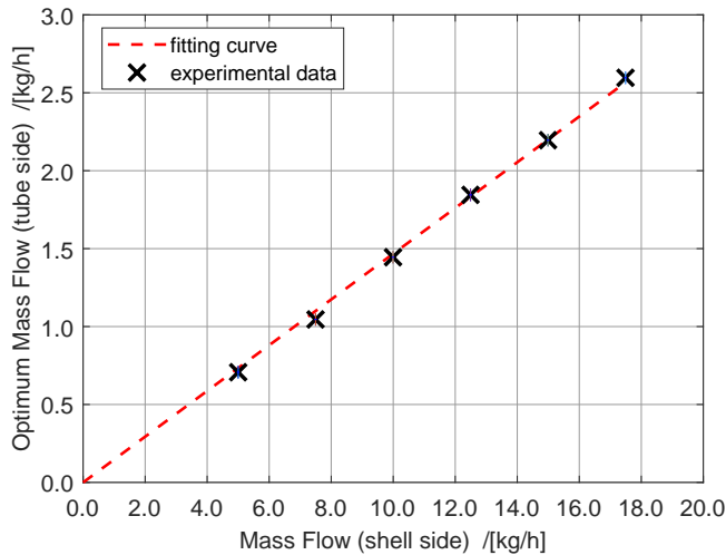
Figure 3.12: The optimum tube side mass flow for each shell side mass flow of the \text{NH}_3\text{-H}_2\text{O} experiments. A clear linear trend can be seen.
