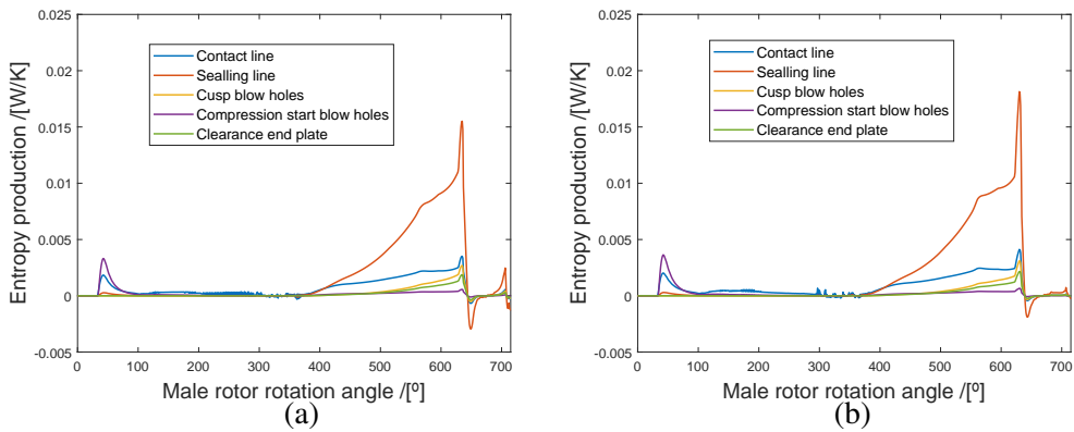
Figure 4.7: \dot{\sigma} for each leakage path in the compressor, 0.6 inlet vapor quality (a) and 0.7 inlet vapor quality (b).
