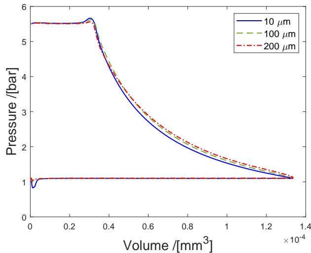
Figure 4.5: P - V diagram for 10 \mu\text{m} (blue solid line), 100 \mu\text{m} (green dashed line) and for 200 \mu\text{m} (red dash-dot line).
