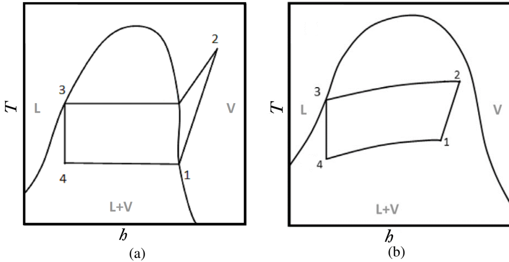
Figure 1.2: Typical Th -diagrams for (a) VCHP, and (b) CRHP utilizing wet compression [12]. The state points correspond to figure 1.1. By compressing in the two state region, superheating is eliminated at the compressor outlet (state point 2).
