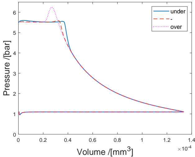
Figure 4.8: P - V diagram for under compression (blue solid line), close to perfect compression (red dashed line) and for over compression (magenta dotted line).
