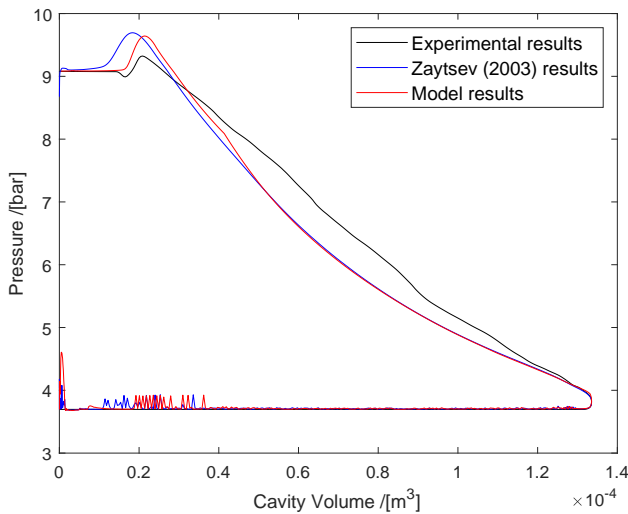
Figure 4.2: Comparison of experimental data from Zaytsev [20], his model and the current model results.
