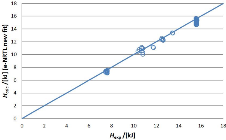
Figure 2.11: Comparison of the experimental data from Rumpf et al. [54] for heat of partial evaporation of the NH 3 -CO 2 -H 2 O mixture and the e-NRTL new fit correlation.
