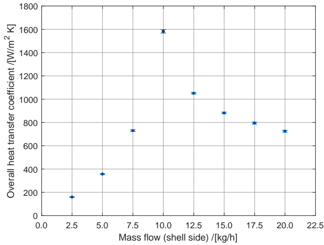
Figure 3.8: Experimental overall heat transfer coefficient based on the tube side area for the water-water experiments. Error bars are included (see section 3.2.1 for details).
