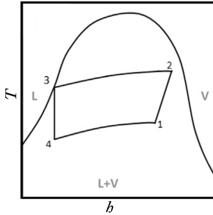
Figure 2.12: Typical temperature-enthalpy diagram for compression-resorption heat pumps. Position 1 indicates the process conditions after the desorber, 2 indicates the conditions at the outlet of the compressor, 3 indicates the conditions at the outlet of the resorber and 4 indicates the conditions after the expansion valve [12].
