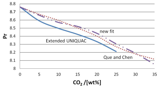
Figure 2.14: Pressure ratio vs CO 2 weight fraction, heating case; waste heat stream is heated from 60 to 105 °C. Results from the extended UNIQUAC model are shown with continuous line, the model of Que and Chen [33] with dotted line, and the new fit with dashed line.
