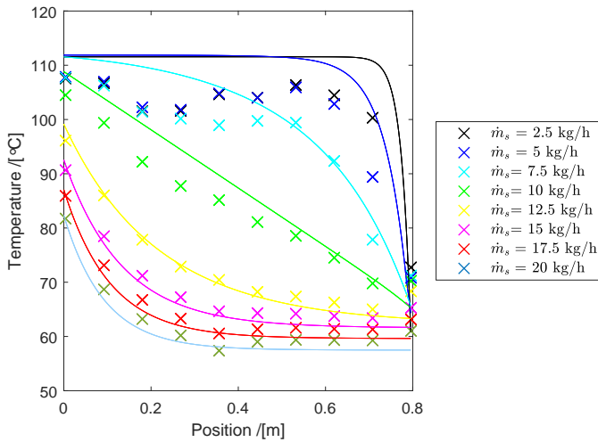
Figure 3.9: Temperatures along the length of the heat exchanger for the water-water experiments. Solid lines are calculated temperatures of the shell side flow with the method proposed by Nefs et al. [74], that is described above, and the marker values are from the temperature sensors along the heat exchanger.
