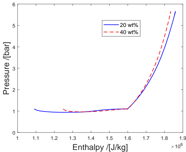
Figure 4.6: Pressure as a function of the local enthalpy, 20 wt.% (blue solid line) and 40 wt.% (red dashed line).
