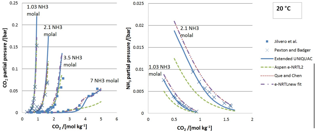
Figure 2.1: Comparison of the experimental data from Pexton and Badger [48] and Jilvero et al. [49] for partial bubble point pressures of \text{CO}_2 and \text{NH}_3 at 20\text{ }^\circ\text{C} with the model correlations.
