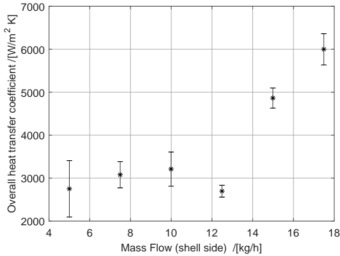
Figure 3.13: The overall heat transfer coefficient for the optimum tube side mass flows of the \text{NH}_3\text{-H}_2\text{O} experiments.
