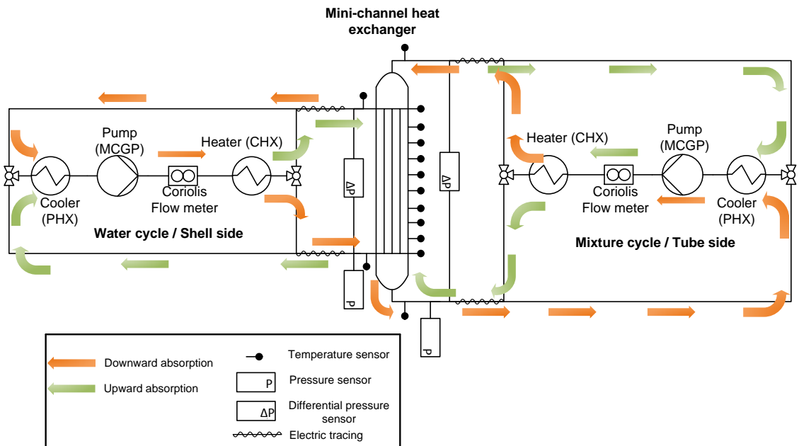
Figure 3.3: A simplified process and instrumentation diagram of the mini-channel test setup. On the left hand side, water is heated up by the means of a coiled heat exchanger and electrical tracing before entering the shell side of the mini-channel heat exchanger. After exiting the heat exchanger the water is subcooled before entering the pump and flow meter. The right hand side is identical, except the mixture enters the tube side of the mini-channel heat exchanger. It is possible to operate the setup with downward absorption (indicated with orange arrows) or upward absorption (indicated with green arrows).
