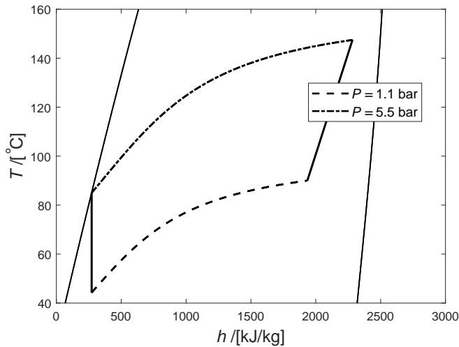
Figure 4.3: T - h diagram of a CRHP, using wet compression, for 30 wt.% \text{NH}_3 . The compression process is entirely in the two phase region from the lower to the higher pressure level. The resorption happens at the higher pressure level, 5.5 bar in this case, then isenthalpic expansion is assumed and the desorption process is at 1.1 bar.
