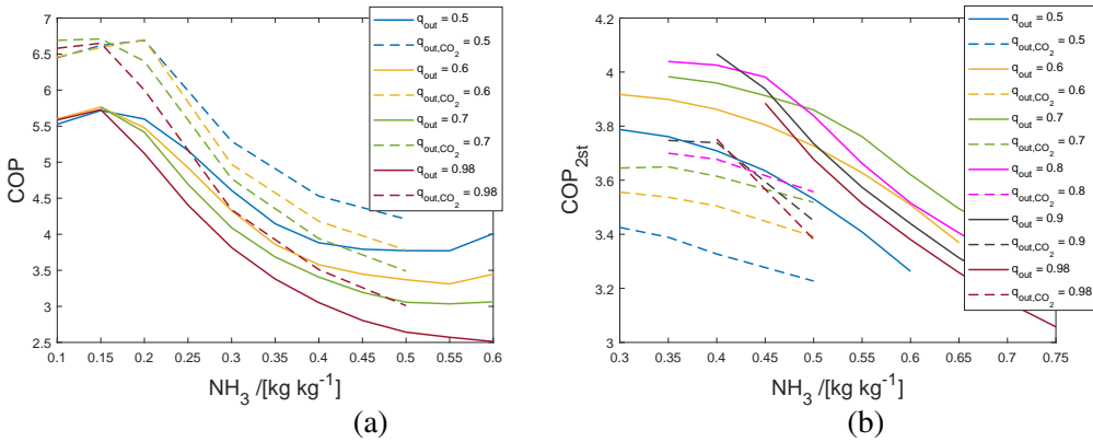
Figure 5.1: COP as a function of the \text{NH}_3 concentration for various compressor outlet vapor qualities when a waste heat stream is heated from 90 to 130 °C (a) and from 60 to 140 °C (b). The solid lines are the results for \text{NH}_3\text{-H}_2\text{O} and the dotted lines with added 5 wt% \text{CO}_2 .
