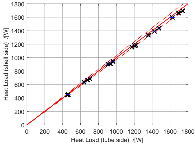
Figure 3.14: The heat load on the shell and tube sides for the \text{NH}_3\text{-H}_2\text{O} experiments. The difference is within 3 % (dotted line) for all the experiments.
