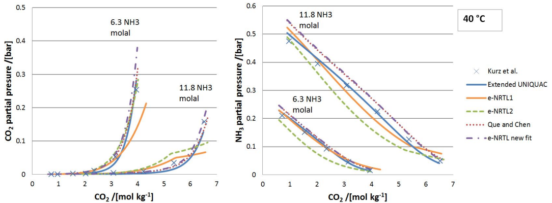
Figure 2.2: Comparison of the experimental data from Kurz et al. [27] for partial bubble point pressures of \text{CO}_2 and \text{NH}_3 at 40\text{ }^\circ\text{C} with the model correlations.
