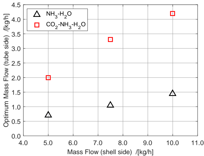
Figure 3.19: Optimum tube side mass flow for the NH 3 -H 2 O and NH 3 -CO 2 -H 2 O experiments for shell side mass flows of 5, 7.5 and 10 kg/h.
