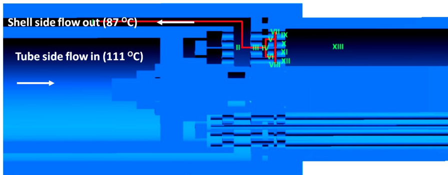
Figure 3.6: Illustration of the shell side outlet of the mini-channel heat exchanger. The temperatures correspond to the measured temperature values of the water-water experiments when the shell side mass flow is kept at 20 kg/h.
