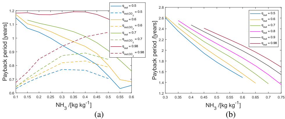
Figure 5.8: The simple payback time taking the cost of \text{CO}_2 into account as a function of the \text{NH}_3 concentration for various compressor outlet vapor qualities, assuming 10 MW thermal output, when a waste heat stream is heated from 90 to 130 °C (a) and from 60 to 140 °C (b). The solid lines are the results for \text{NH}_3\text{-H}_2\text{O} and the dotted lines with added 5 wt% \text{CO}_2 .
