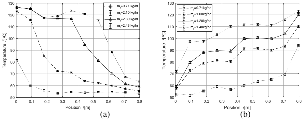
Figure 3.23: Temperature values along the mini-channel for a shell side mass flow of 5 kg/h, for downward absorption of the \text{NH}_3\text{-CO}_2\text{-H}_2\text{O} mixture (a), and upward absorption of the \text{NH}_3\text{-CO}_2\text{-H}_2\text{O} mixture (b). Error bars are included (see section 3.2 for details). The lines serve as visual guidelines for the reader.
