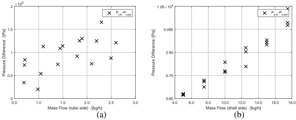
Figure 3.15: Pressure drop over the mini-channel heat exchanger on the tube side (NH 3 -H 2 O side) (a), and the shell side (water side) (b).
