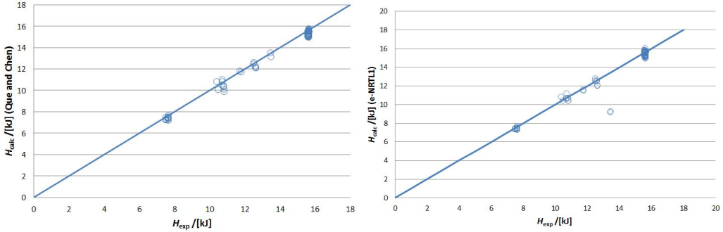
Figure 2.9: Comparison of the experimental data from Rumpf et al. [54] for heat of partial evaporation of the NH 3 -CO 2 -H 2 O mixture: (left) Que and Chen [33] and (right) e-NRTL1 correlation.
