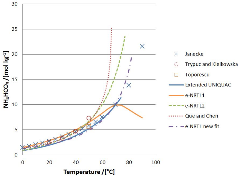
Figure 2.6: Comparison of the experimental data from Janecke [43], Trypuc and Kielkowska [51] and Toporescu [52] for solubility of \text{NH}_4\text{HCO}_3 in water with the model predictions.
