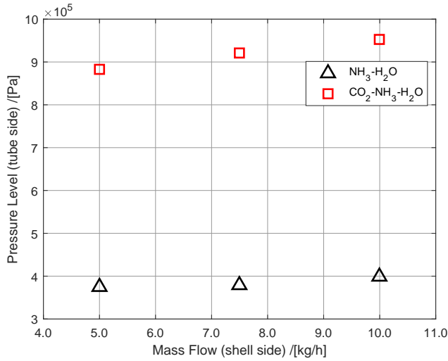
Figure 3.20: Pressure levels for the \text{NH}_3\text{-H}_2\text{O} and \text{NH}_3\text{-CO}_2\text{-H}_2\text{O} experiments for shell side mass flows of 5, 7.5 and 10 kg/h.
