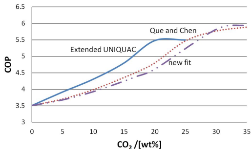
Figure 2.15: COP vs CO 2 weight fraction, 0.3 to 25 bar pressure limit; waste heat stream is heated from 60 to 105 °C. Results from the extended UNIQUAC model are shown with continuous line, the model of Que and Chen [33] with dotted line, and the new fit with dashed line.
