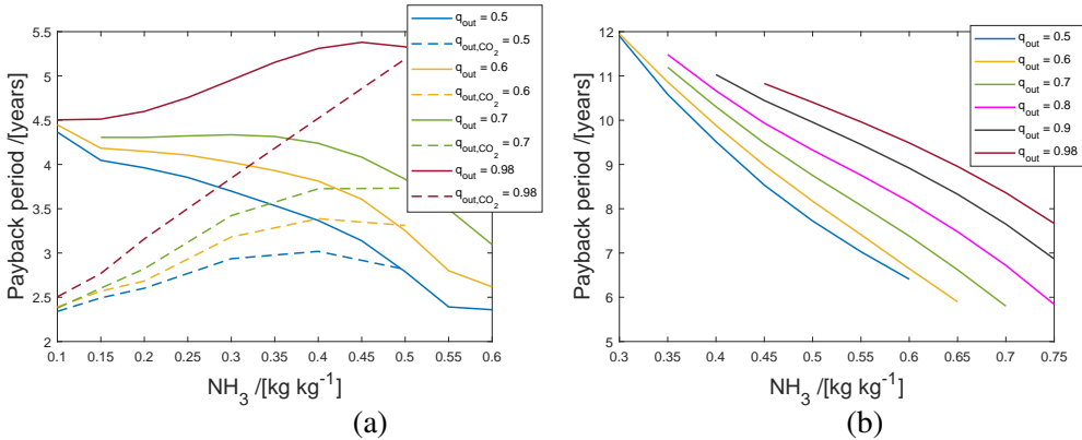
Figure 5.5: The simple payback time as a function of the NH 3 concentration for various compressor outlet vapor qualities, assuming 1 MW thermal output, when a waste heat stream is heated from 90 to 130 °C (a) and from 60 to 140 °C (b). The solid lines are the results for NH 3 -H 2 O and the dotted lines with added 5 wt% CO 2 .
