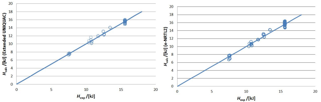
Figure 2.10: Comparison of the experimental data from Rumpf et al. [54] for heat of partial evaporation of the NH 3 -CO 2 -H 2 O mixture: (left) extended UNIQUAC and (right) e-NRTL2 correlation.
