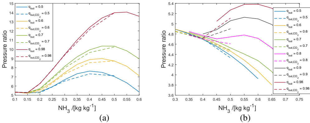
Figure 5.2: Pressure ratio as a function the \text{NH}_3 concentration for various compressor outlet vapor qualities when a waste heat stream is heated from 90 to 130 °C (a) and from 60 to 140 °C (b). The solid lines are the results for \text{NH}_3\text{-H}_2\text{O} and the dotted lines with added 5 wt% \text{CO}_2 .
