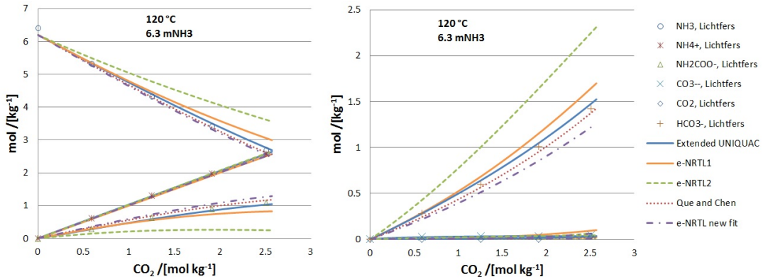
Figure 2.8: Comparison of the experimental from Lichtfers [53] data for speciation at 120 °C and molality of 6.3 mol/kg \text{NH}_3 with the model correlations.
