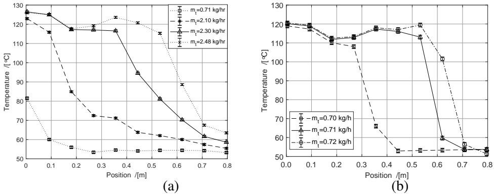
Figure 3.22: Temperature results from the sensors located along the shell side of the mini-channel heat exchanger for a shell side mass flow of 5 kg/h, for the \text{NH}_3\text{-CO}_2\text{-H}_2\text{O} mixture (a), and the \text{NH}_3\text{-H}_2\text{O} mixture (b). Error bars are included (see section 2 for details). The lines serve as visual guidelines for the reader.
