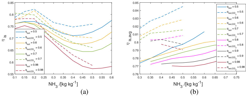
Figure 5.3: \eta_{is} as a function of the \text{NH}_3 concentration for various compressor outlet vapor qualities when a waste heat stream is heated from 90 to 130 °C (a) and from 60 to 140 °C (b). The solid lines are the results for \text{NH}_3\text{-H}_2\text{O} and the dotted lines with added 5 wt% \text{CO}_2 .
