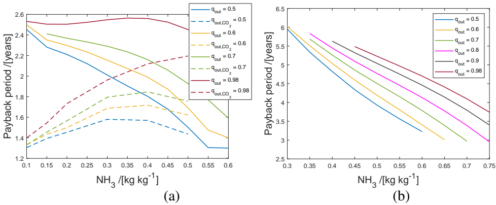
Figure 5.6: The simple payback time taking the cost of CO 2 into account as a function of the NH 3 concentration for various compressor outlet vapor qualities, assuming 1 MW thermal output, when a waste heat stream is heated from 90 to 130 °C (a) and from 60 to 140 °C (b). The solid lines are the results for NH 3 -H 2 O and the dotted lines with added 5 wt% CO 2 .
