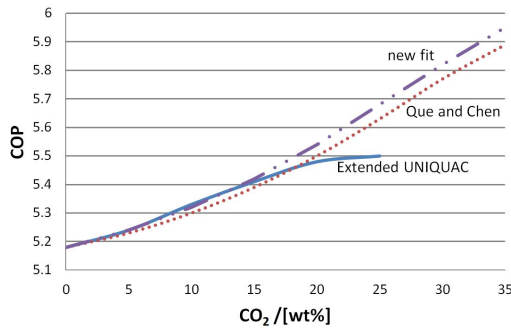
Figure 2.13: COP vs CO 2 weight fraction, heating case; waste heat stream is heated from 60 to 105 °C. Results from the extended UNIQUAC model are shown with continuous line, the model of Que and Chen [33] with dotted line, and the new fit with dashed line.
