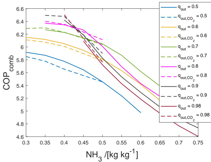
Figure 5.4: \text{COP}_{comb} as a function of \text{NH}_3 concentration for various compressor outlet vapor qualities when a waste heat stream is heated from 60 to 140 °C. The solid lines are the results for \text{NH}_3\text{-H}_2\text{O} and the dotted lines with added 5 wt% \text{CO}_2 .
