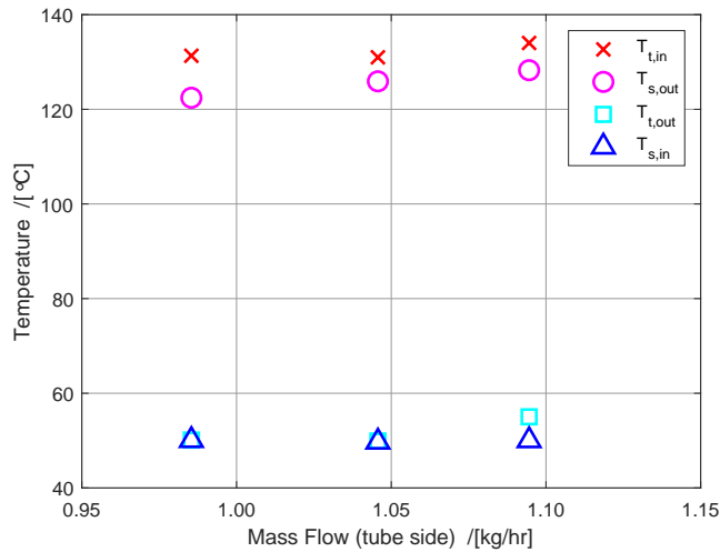
Figure 3.11: In- and outlet temperatures for the \text{NH}_3\text{-H}_2\text{O} experiments at various tube side mass flows when the shell side mass flow is kept constant at 7.5 kg/h.
