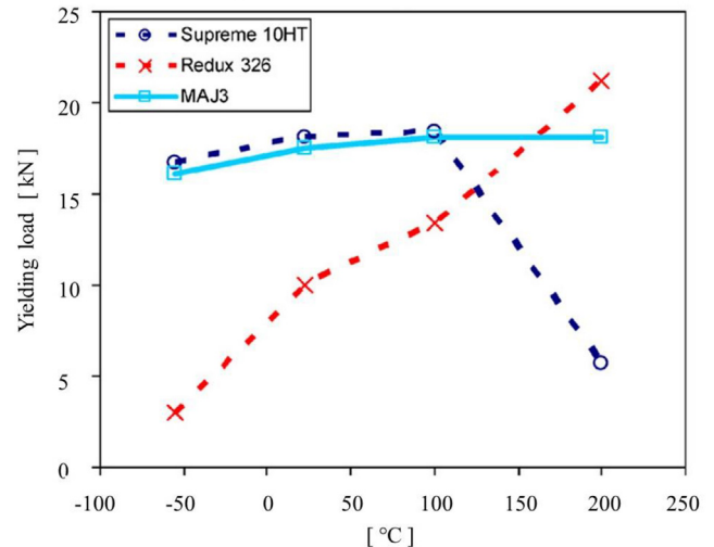
Fig. 8. Yielding load of functionally graded CFRP-Titanium DLJs over a wide range of temperature [46].
