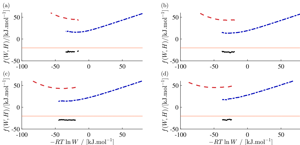
Figure 6. (Colour online) Two-dimensional overlapping distribution method (Equation (5)) applied to the TIP4P-EW liquid water model in the NVT ensemble with a void fraction of \phi = 0.45 , based on the computed coexistence densities at T = 300 K. The sampled hydrogen bond count in each subfigure equals: (a) H = 0 ; (b) H = 1 ; (c) H = 2 ; (d) H = 3 . In all sub-figures: (—) f_1(W, H) , (— · —) f_0(W, H) , (····) \mu_{WTPI}^{ex} , (—) f_0(W, H) - f_1(W, H) .
