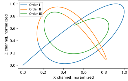
Figure 10: Theoretical constellation
