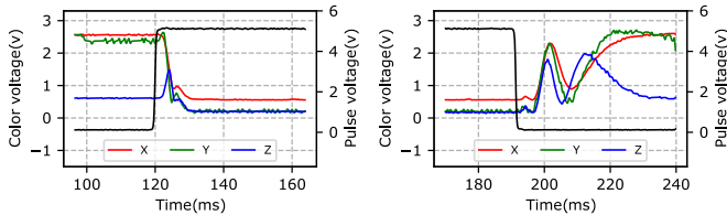
Figure 24: Empirical response for four slow LCs
