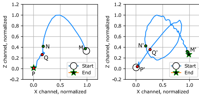
Figure 25: Constellations for four slow LCs
