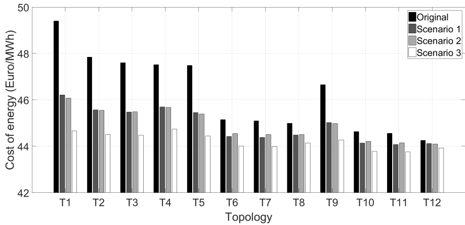
Figure 3.18: Comparison of capital cost of energy for twelve topologies.
