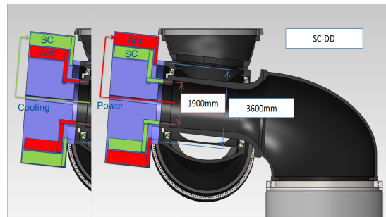
Figure 2.31: Two possibilities of arranging the superconducting field winding and the copper armature winding in the INNWIND.EU nacelle concept. The superconducting field winding will rotate if placed outside. The axle hollow can be used as a channel for placing pipes connecting rotating cryocoolers' cold heads to stationary compressors. [85]
