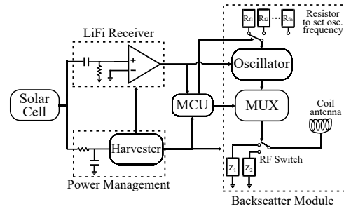
Figure 7: Block diagram of LeakageScatter battery-free tag.
