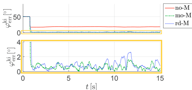
Fig. 6. Relative orientation error \varphi_{\text{err}}^{ki} between the orientation \mathbf{q}_{b_i}^r of segment i and the orientation \mathbf{q}_{b_k}^r of segment k .
