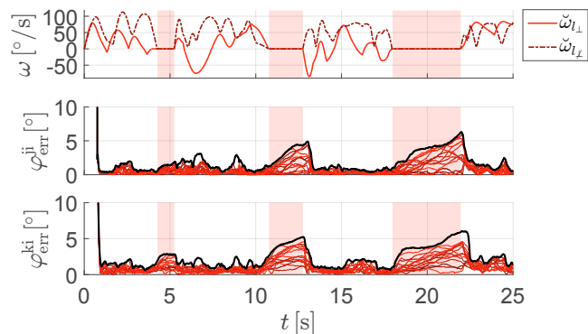
Fig. 7. Motion and estimation error for the random movement with non-observable intervals. The red areas highlight the intervals where \omega_{l_\perp}^{b_j} and \omega_{l_x}^{b_j} are zero.
