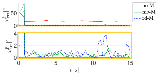
Fig. 5. Relative orientation error \varphi_{\text{err}}^{ji} between the orientation \mathbf{q}_{b_i}^r of segment i and the orientation \mathbf{q}_{b_j}^r of segment j .
