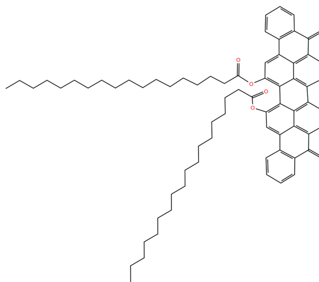
Figure 1. 2D molecular structure of Violanthrone-78. Polycyclic aromatic core, polar heteroatoms, and two side chains are shown.
