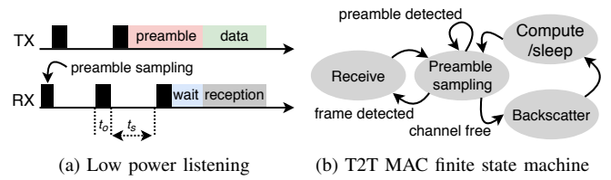
Fig. 7. Schematic representation of the proposed MAC protocol. Fig. 7a: low-power listening diagram (for t_s and t_o see Table IV); Fig. 7b: MAC state machine (for both transmitter and receiver).
