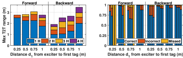
(a) T2T multi-hop range at hop H (b) Received frame distribution
