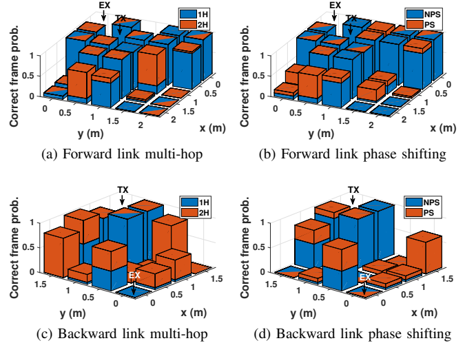
Fig. 10. Backscatter T2T network phase cancellation experiment. EX and TX mark the positions of the exciter and transmitter, respectively. ( N )/ PS : (no) phase shifting. Fig. 10a and 10b: forward link. Both methods yield comparable results. Fig. 10c and 10d: backward link. Multi-hop is superior in network coverage. Note: 1H and NPS is the same case.
