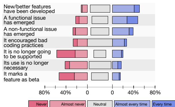
Figure 3: Motivations to react to deprecation according to API consumers' experience, by decreasing frequency
