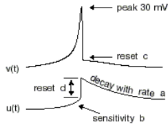
Fig. 1. Izhikevich Spike
