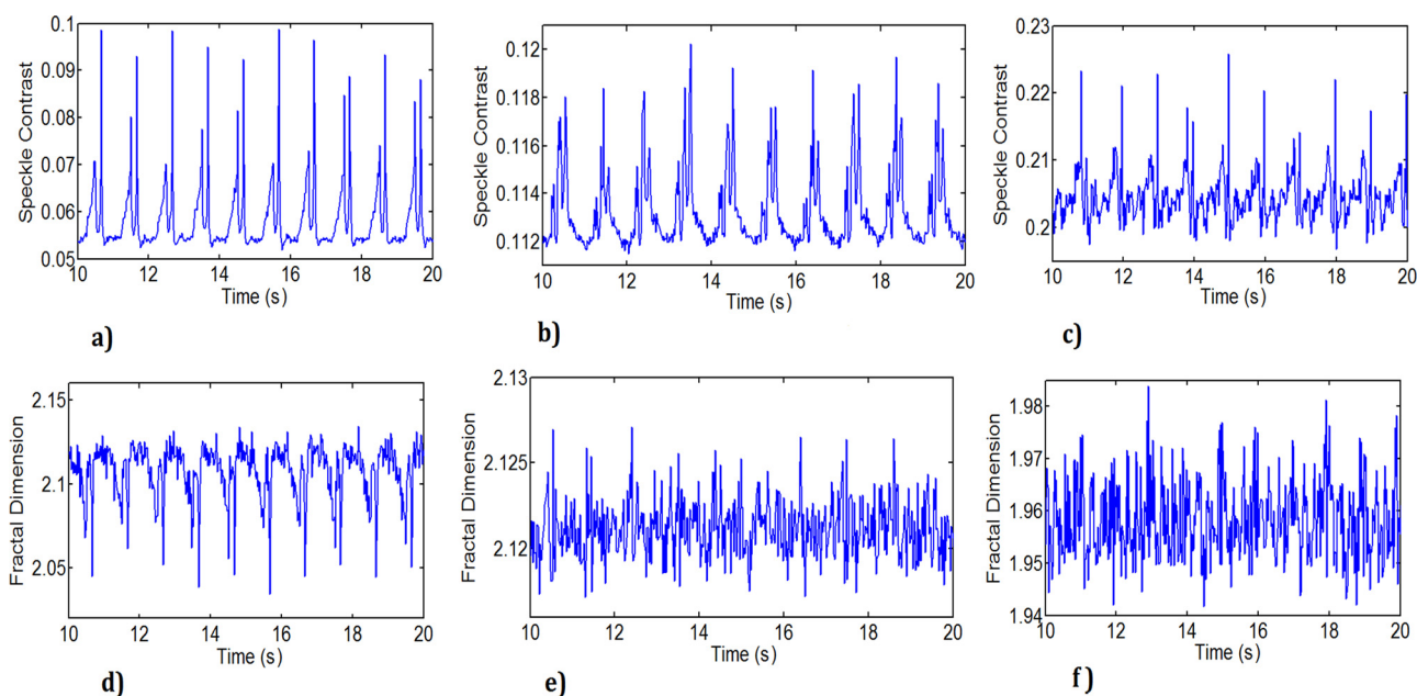
FIG. 4. The time series signal measured for pulsatile flow in the rectangular flow channel with different top membranes. (a) Glass membrane, images analyzed, with speckle contrast. (b) 1 mm thick Delrin membrane, images analyzed, with speckle contrast. (c) 2 mm thick Delrin, images analyzed, with speckle contrast. (d) Glass membrane, images analyzed, with fractal dimension. (e) 1 mm thick Delrin membrane, images analyzed, with fractal dimension. (f) 2 mm thick Delrin membrane, images analyzed, with fractal dimension.
