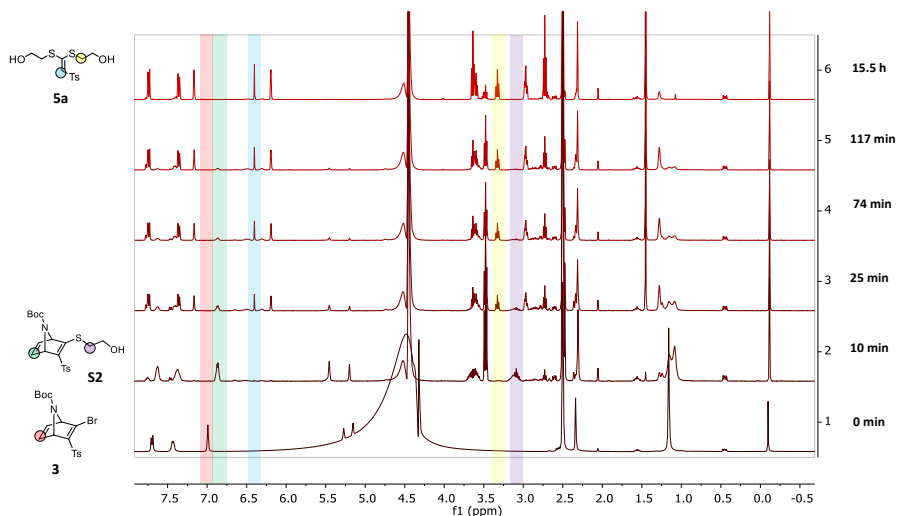
Figure S5.5. 1 H-NMR (399.7 MHz, 298 K in 50%DMSO/(PB8.2+D 2 O) spectra of reaction between azanorbornadiene bromo sulfone 3 and β-mercaptoethanol at room temperature. Spectrum 1 shows that only azanorbornadiene bromo sulfone 3 (1.8 mg, 0.004 mmol, 1 eq) was in the solution at t = 0 min. Spectrum 2 to Spectrum 6 show the mixture at different time points after adding β-mercaptoethanol
