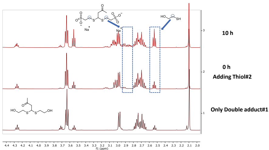
Figure S3.3. 1 H-NMR (399.7 MHz, 298 K in D 2 O / PB8.2, 4 drops of D 2 O in 1 mL PB8.2) monitoring of dynamic exchange between thiol#1-alkynone double adduct and sodium 2-mercaptoethanesulfonate (thiol#2) in sodium phosphate buffer (100 mM, pH=8.2) at room temperature.
