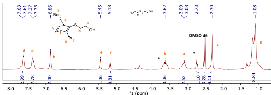
Figure S5.2. ^1\text{H-NMR} (399.7 MHz, 298 K in \text{DMSO-d}_6 ) spectrum of the single BME conjugation product S2 .
