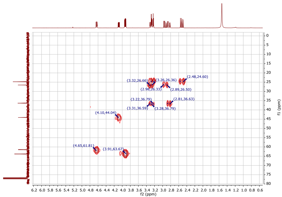
Figure S2.6. ^1\text{H} - ^{13}\text{C} HSQC at 298 K in \text{CDCl}_3 spectrum of the aliphatic region of the oxidation product \text{S}_1 .
