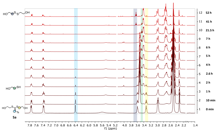
Figure S5.7. ^1\text{H-NMR} (399.7 MHz, 298 K in 50%DMSO/(PB8.2+D 2 O)) spectra of reaction between bis-thiolated vinyl sulfone product 5a and DTT at room temperature. Spectrum 1 shows that only 5a (3.0 mg, 0.009 mmol, 1 eq) was in the solution at t = 0 min. Spectrum 2 to Spectrum 12 show the mixture at different time points after adding DTT (13.9 mg, 0.09 mmol, 10 eq.) into the solution. Green highlights represent the characteristic peaks of BME. Blue and yellow highlights represent the characteristic peaks of 5a . Grey highlight represents the characteristic peak of oxidized 2-mercaptoethanol.
