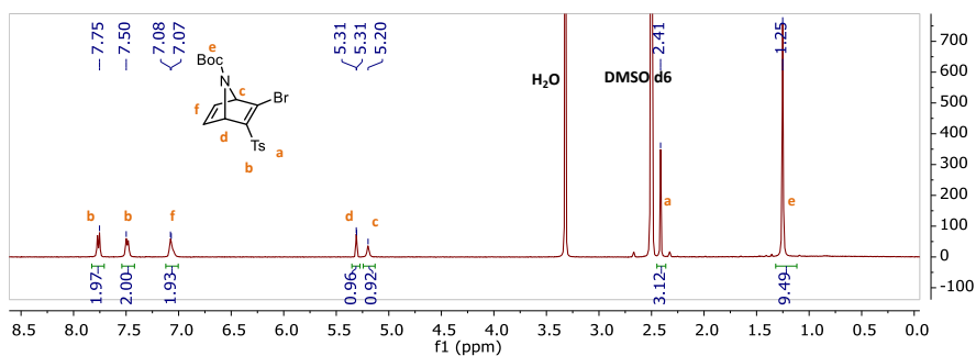
Figure S5.1. ^1\text{H-NMR} (399.7 MHz, 298 K in \text{DMSO-d}_6 ) spectrum of Azanorbornadiene bromo vinyl sulfone 3 .
