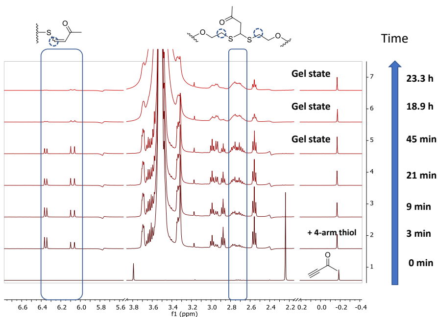
Figure S3.4. 1 H-NMR (399.7 MHz, 298 K in D 2 O / PB8.2, 15 \mu L D 2 O in 585 \mu L PB8.2) monitoring of single addition and double addition during thiol-alkynone double addition hydrogel formation between 3-butyne-2-one and 4-arm PEG thiol.
