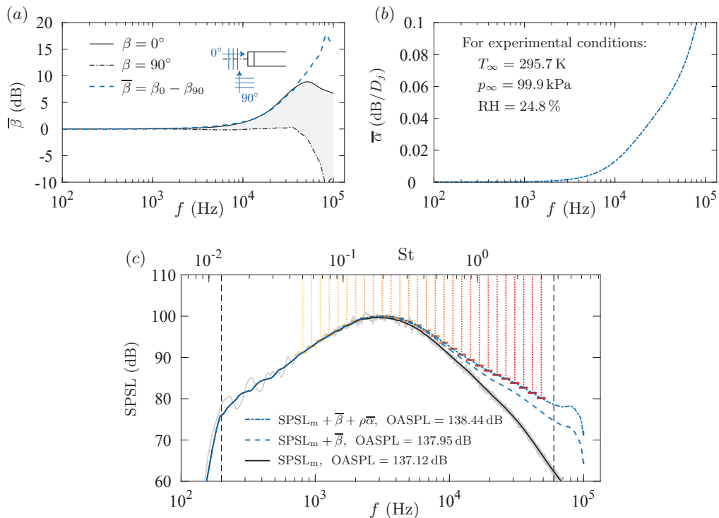
FIGURE 6. (a) Method for calculating free-field microphone correction. (b) Sample atmospheric absorption correction curve \bar{\alpha} . (c) Sound pressure spectrum level at (x, r)/D_j = (35, 39) . The OASPL values provided correspond to spectral integrations between the vertical dashed lines at f = 200 Hz and f = 60 kHz. Twenty-eight logarithmically-spaced lines in the range 0.05 \leq \text{St} \leq 3 identify the centre Strouhal numbers for the analysis described in § 3.1.
