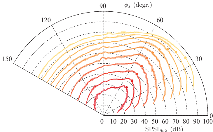
FIGURE 14. \text{SPSL}_{b,S}(x,r;St_b) polar patterns at \rho_s^* = 60D_j for 10 Strouhal numbers, corresponding to bin b = 1 : 3 : 28 . The solid thick lines identifies the average polar pattern; envelopes represent the spread from the root-mean-square of data points while subsequent polar patterns are offset by -5 dB (from yellow-to-red).
