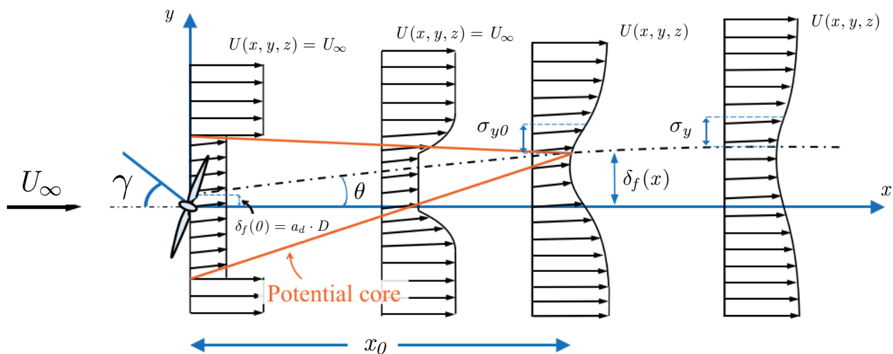
Figure 2. Schematic overview of the wake of a yawed turbine (a negative misalignment angle is shown). Originally taken from Bastankhah and Porté-Agel [44] and modified by Doekemeijer et al. [14].
