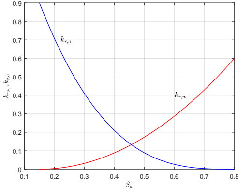
Figure 3.1: Corey's relative permeabilities with k_{r,w}^0 = 0.6 , k_{r,o}^0 = 0.9 , n_w = 2 , n_o = 3 , S_{wir} = 0.15 , S_{or} = 0.2 .
