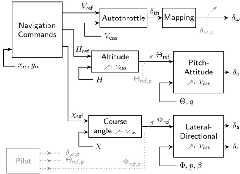
Figure 15 : Control architecture for fully automated flight (mode (iii)), and augmented flight (mode (ii)), indicated in gray.
