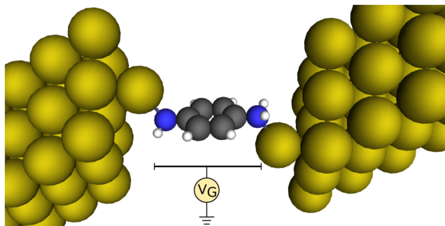
FIG. 8. Scheme showing the Au-BDA-Au junction and the gate applied on the molecule.
