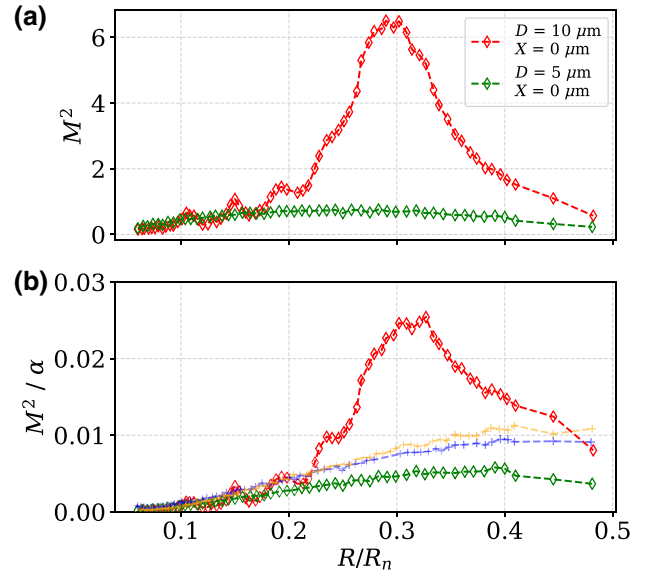
FIG. 8. (a) Excess noise M^2 and (b) M^2 / \alpha for low-frequency pixels with different stem diameters. In (a), data are shown for the X = 0 , D = 10 \mu\text{m} (red) and X = 0 , D = 5 \mu\text{m} (green) devices. In (b), also the data for the X = 5 \mu\text{m} (blue) and X = 10 \mu\text{m} (yellow) devices are shown as a reference.
