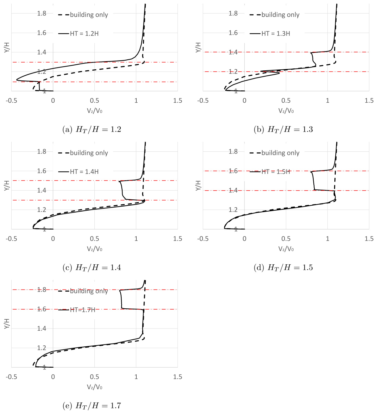
Figure 3: Plot of the y position normalized with the building height H against velocity V_z normalized with the reference free stream velocity(6m/s). The profiles are shown at the rotor position. Each result is compared with the case of no turbine. The turbine location is indicated by the dotted red lines. The location of the turbine along the free stream direction is at the centre of the building.
