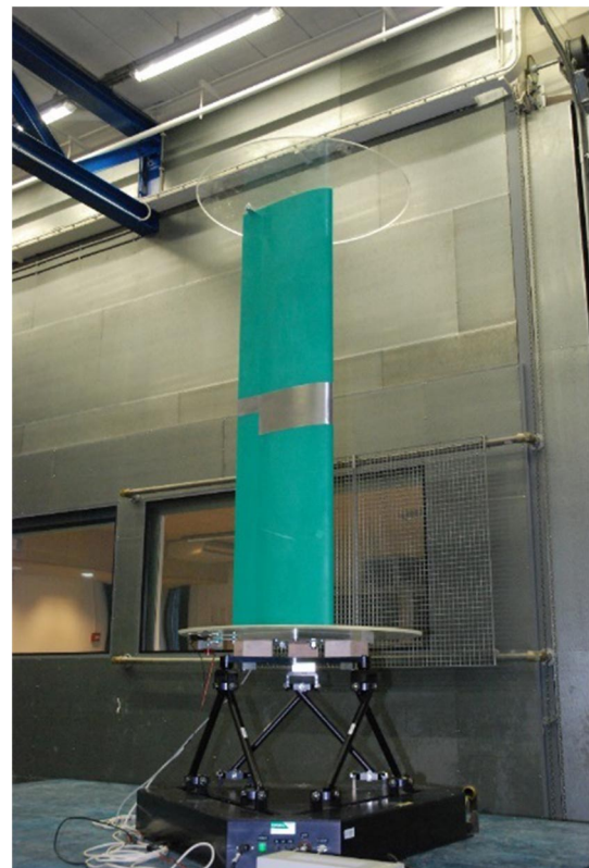
Fig. 2 The wing model on the 6-DOF platform.
