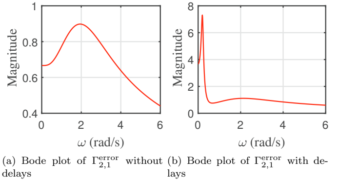
Fig. 3. Error transfer function for \lambda = 1.0 , q_1 = 0.8 , q_3 = 0.5 , q_4 = 0.4 , \tau = 0.25 s, \delta_{s,i} = 0.02 s, \delta_{p,i} = 0.1 s, \delta_{l,i} = 0.1 \times i s.
