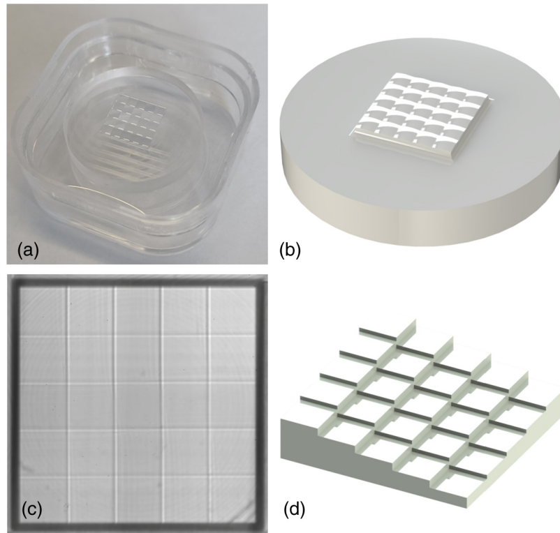
Fig. 4 (a) Microlenses array used in the prototype of the white light interferometer. The array contains 25 plano-convex microlenses of 1.8 mm by 1.8 mm pitch each. (b) CAD design of the micro-lenses array. (c) Manufactured optical phase mask of 25 steps and 160 nm height difference between consecutive steps. (d) CAD design of the optical phase mask where the height difference has been exaggerated for visualization purposes.
