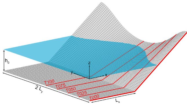
Fig. 2. Problem geometry Zelt test case. L_y is the half wavelength of the sinusoidal bay; L_s is the width of the shelf; Txxx indicates the number of the line where the run-up heights are recorded in Fig. 3(a).
