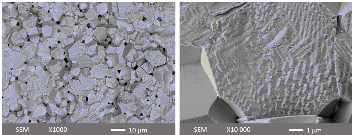
Figure 1. (SEM) images of a fractured 0.6\text{BiFeO}_3\text{-}0.2\text{PbTiO}_3\text{-}0.3\text{SrTiO}_3 ceramic after sintering (acceleration voltage—5 kV).
