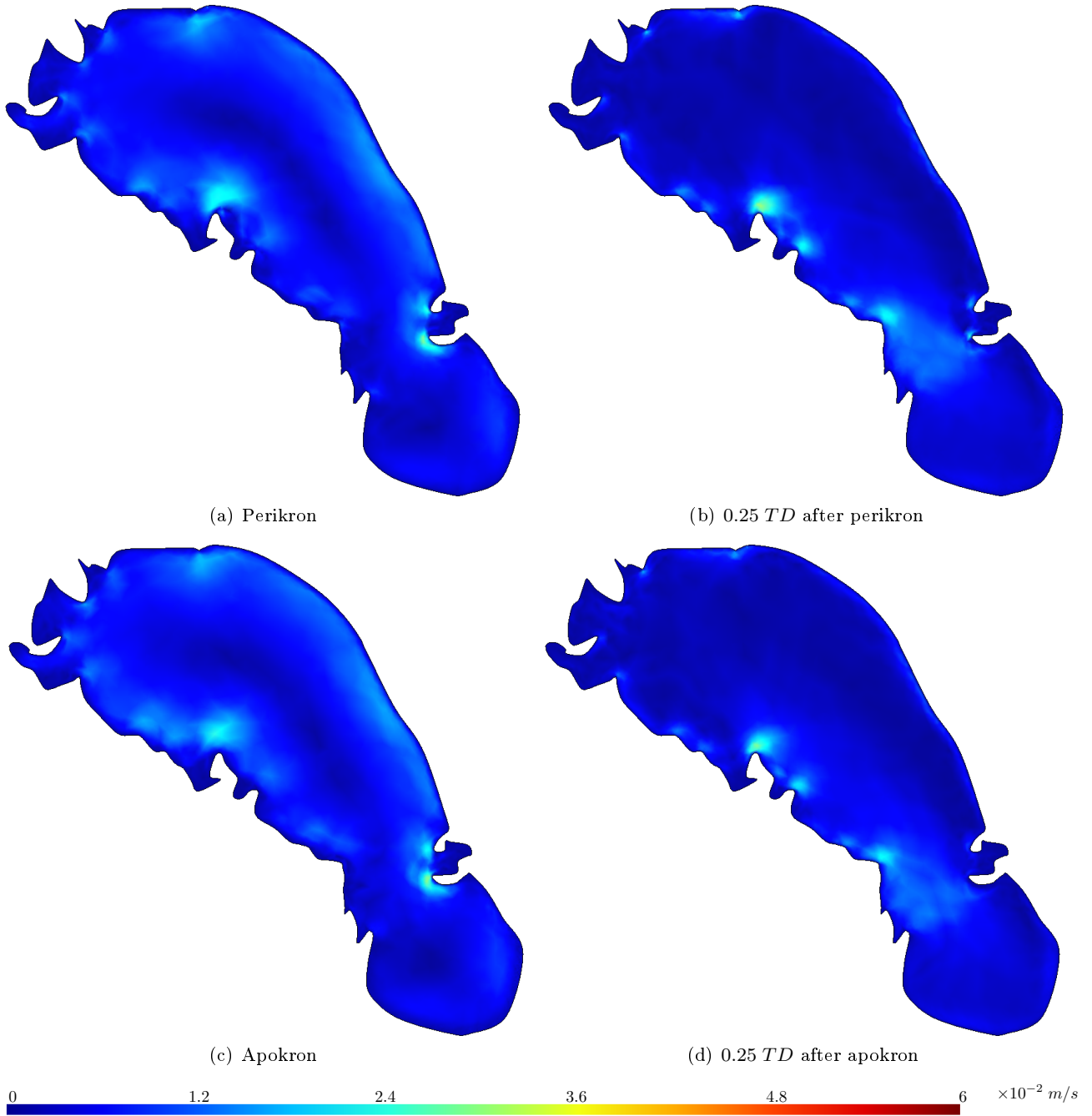
Fig. 11 Tidal current magnitude (in ms^{-1} ) in Ontario Lacus with bathy B implemented at (a) Perikron, (b) 0.25 TD after Perikron, (c) Apokron and (d) 0.25 TD after Apokron. The current magnitude is maximum nearshore, at area E, and is significantly large at area G
