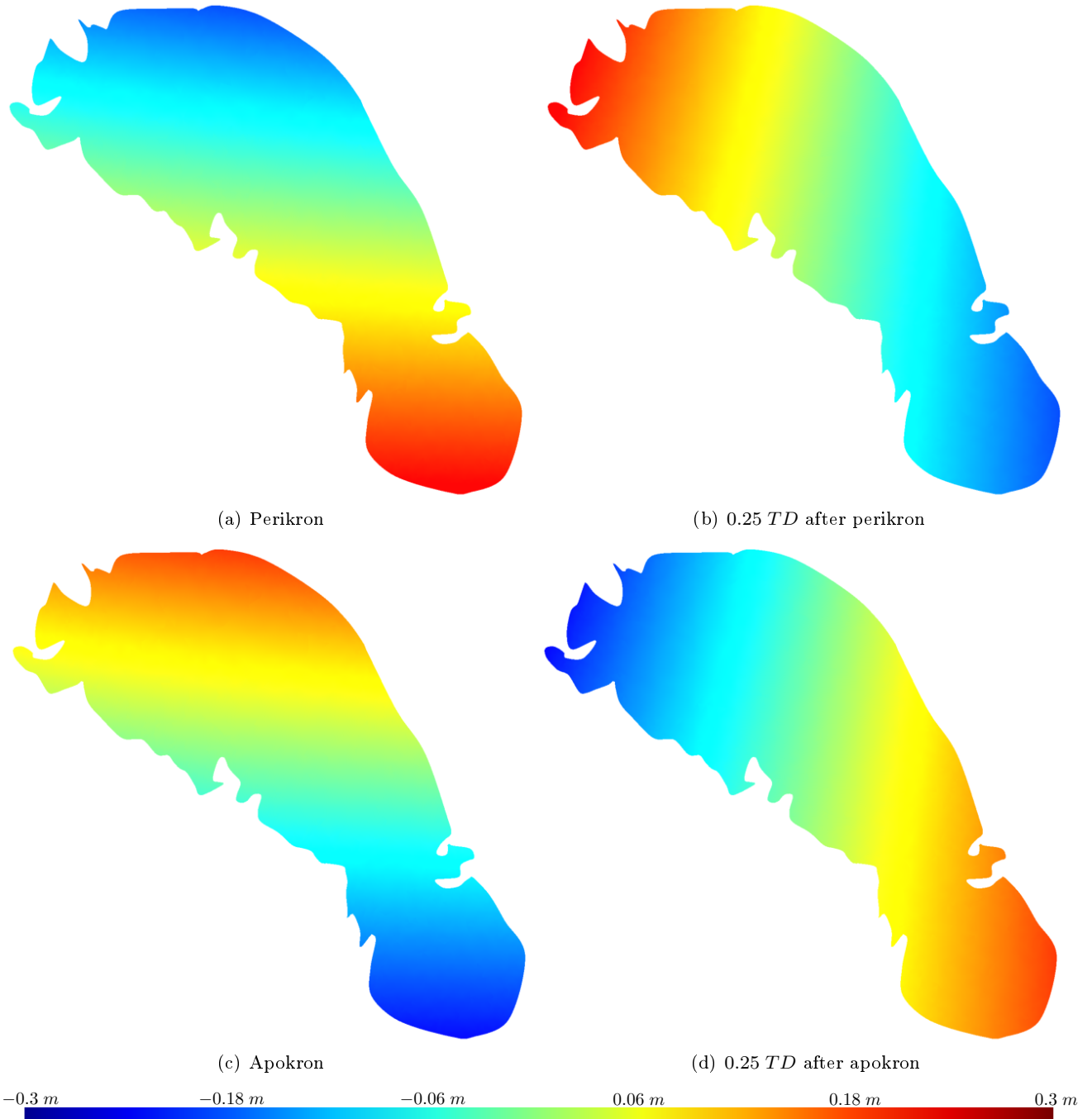
Fig. 6 Surface elevation (in meters) in Ontario Lacus at (a) Perikron, (b) 0.25 TD after Perikron, (c) Apokron and (d) 0.25 TD after Apokron with bathy C implemented. The tide is high in the southern part at perikron and rotates clockwise with an exact period of 1 Titan day. The maximum/minimum surface elevation respectively occurs 0.11 TD before perikron/apokron, in the south
