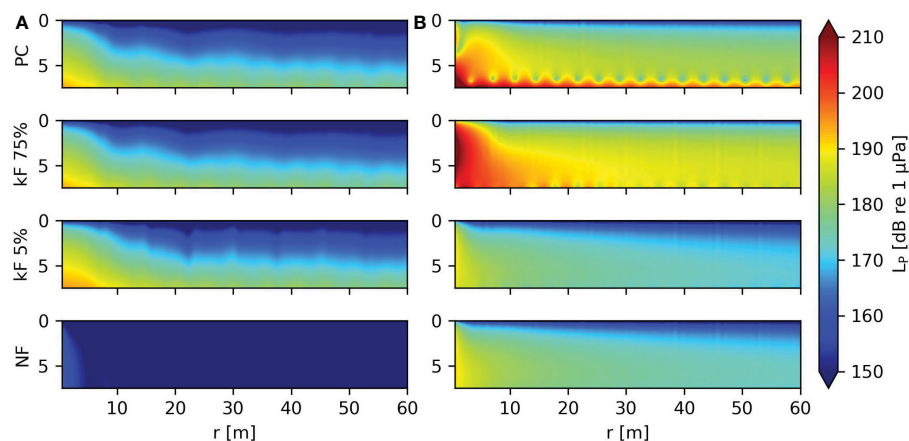
FIGURE 7 Figure (A, B) show the sound pressure levels in dB versus depth and height in the fluid for a harmonic 1 MN force at 25 Hz and 125 Hz respectively.
