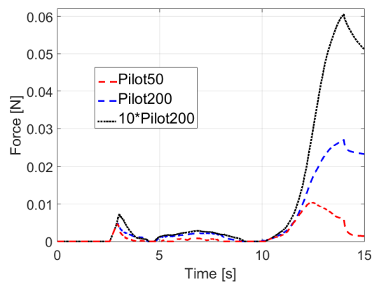
Figure 9: Contact forces caused by guidewires of different bending stiffness
