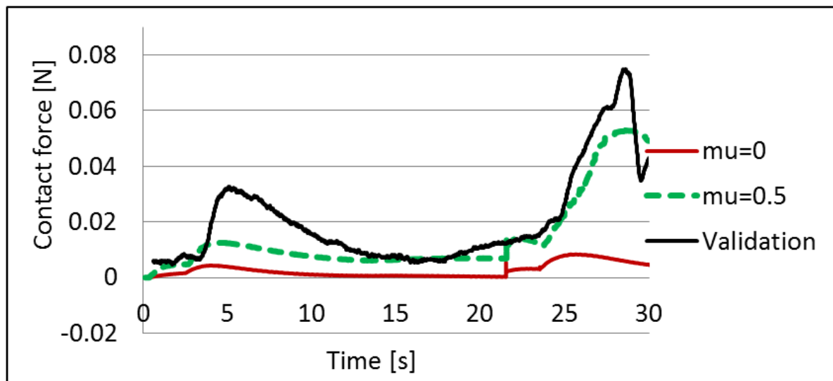
Figure 9: Comparing the transition of applied forces between guidewire and vasculature wall along y-axis in simulation (n=200) with different friction coefficient and the validation experiment: Amplatz guidewire.
