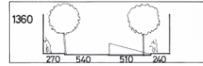
One-sided parking, perpendicular r_p = 0.4 parking lots/m ( b > 15.60\text{m} )
