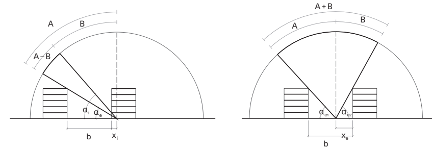
17 Contribution of the sky to the intensity in the interior, A - B (left); and exterior, A + B (right).
