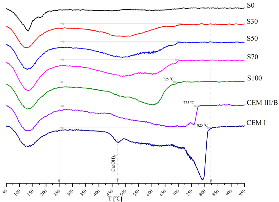
b) DTG curves for carbonated powders (after 180 days of carbonation).
