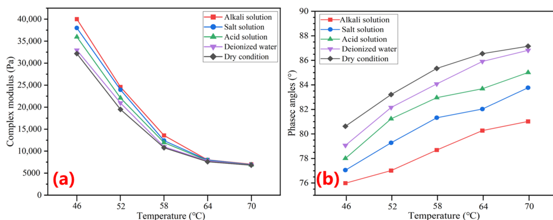
Figure 16. The G^* (a) and \delta (b) of asphalt binders retrieved from noncapsule asphalt concrete after different solution treatments.
