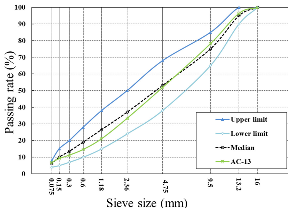
Figure 3. The aggregate gradation curve of AC-13 bituminous mixtures [42–44].
