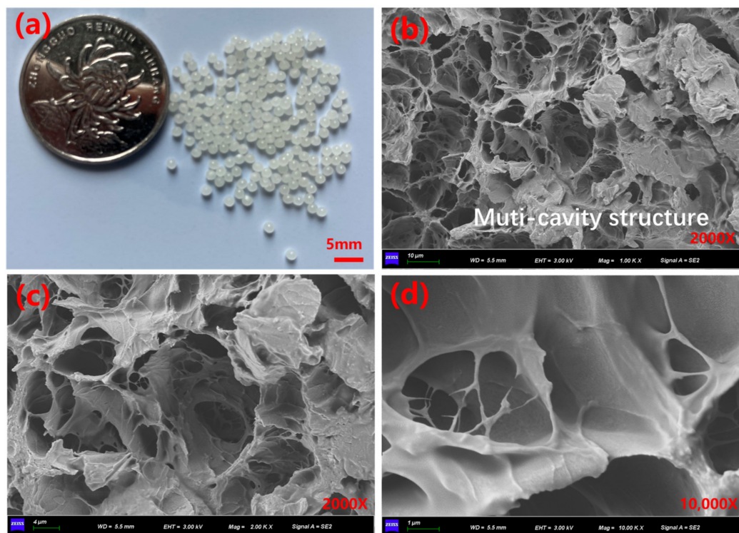
Figure 6. (a) Appearance image of polymer capsules; (b–d) inner structure of capsules at varying magnification levels.
