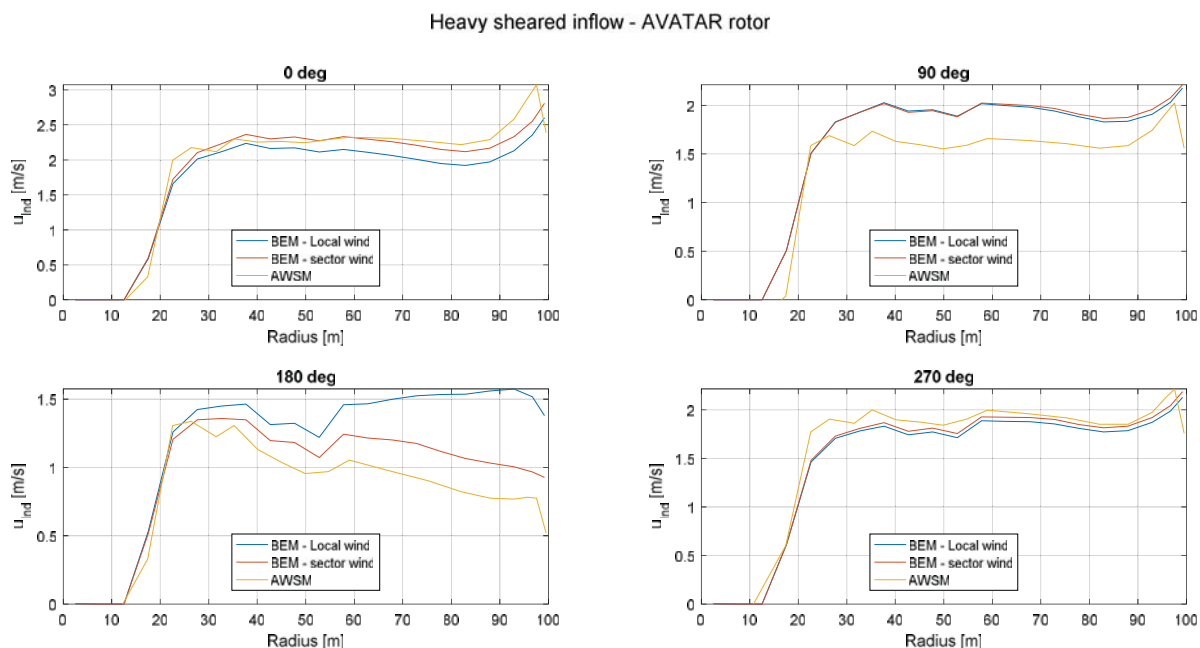
Figure 10 Calculation with ECN's Aeromodule for the AVATAR rotor under heavy shear: induced velocity calculated with element approach and local or sector wind compared with AWSM results for 4 azimuth angles.
