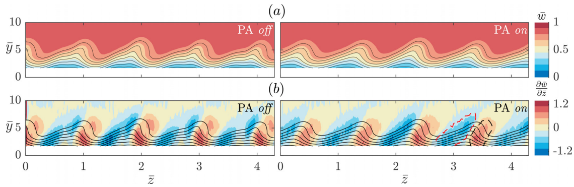
FIG. 9. (a) Time-averaged velocity fields \bar{w} and (b) spanwise gradient of mean flow \partial\bar{w}/\partial\bar{z} for the DRE- H case. Plane location is at x/c_x = 0.225 , and black iso-lines illustrate \bar{w} , ten levels from 0 to 0.9. The regions outlined by dashed lines in (b) are based on thresholds of -0.23 and 0.5 .
