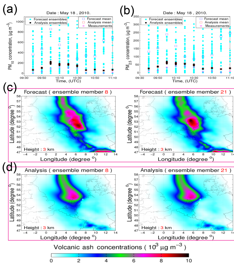
Figure 2. Assimilation effect from 09:40 to 11:10 UTC, 18 May 2010. (a, b) Volcanic ash concentrations of PM_{10} and PM_{2.5} at measurement locations. (c, d) Volcanic ash ensemble state (ensemble member 8 and 21) of forecast and analysis at 11:10 UTC. The measurements, ensembles and mean of forecast and analysis are shown in (a, b). In (c, d), the area of interest is marked as red rectangular in Fig. 1a. The evaluation height is chosen at 3 km since the measurements are taken at altitudes around this height, see Sect. 2.2.
