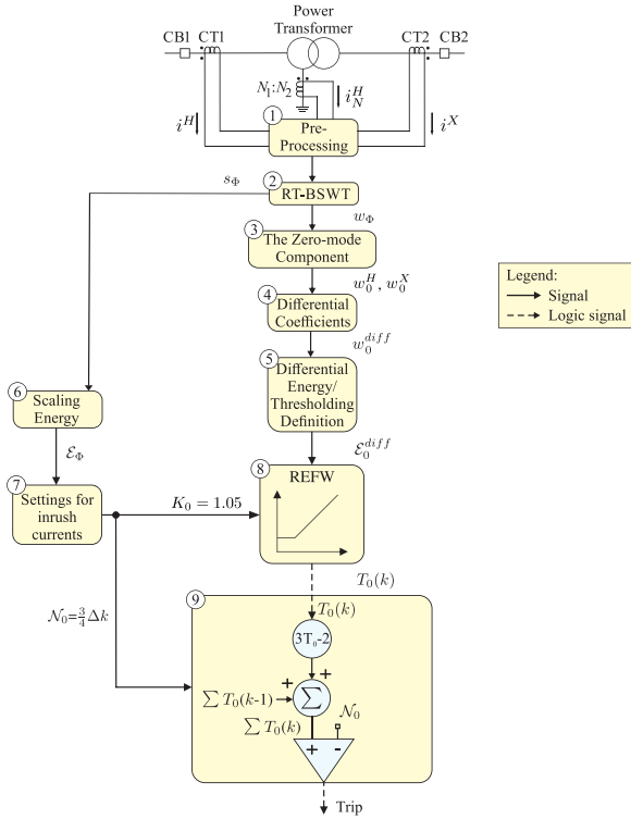
Fig. 1. The proposed Clarke-wavelet-based differential protection.
