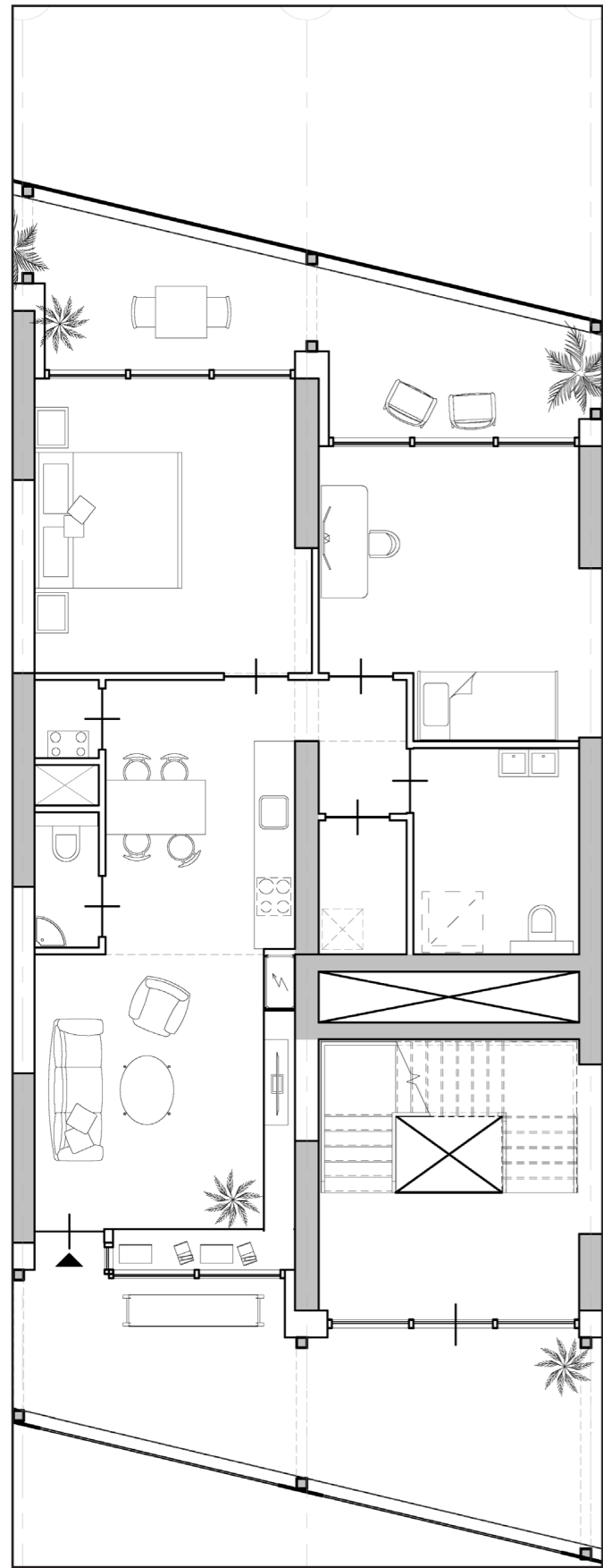
Corner apartment 1:100
