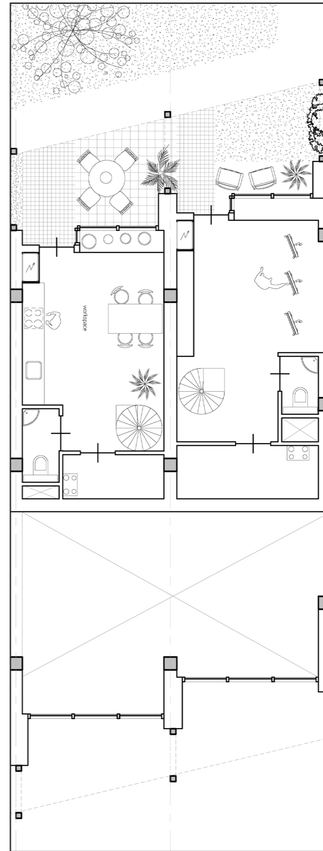
Atelier dwellings 1:100
