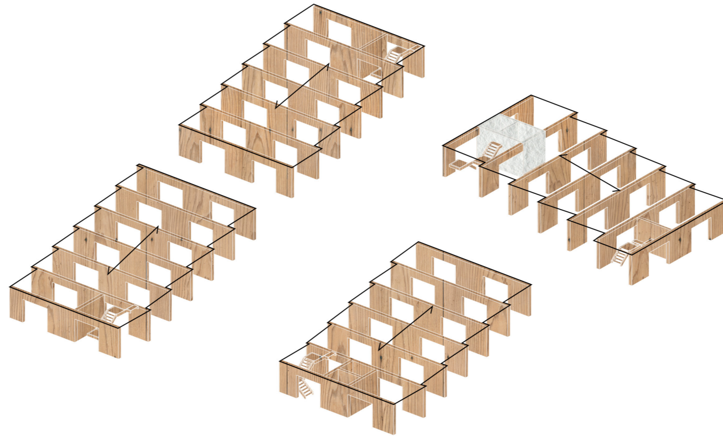
2nd-12th floor - CLT slabs with concrete core
